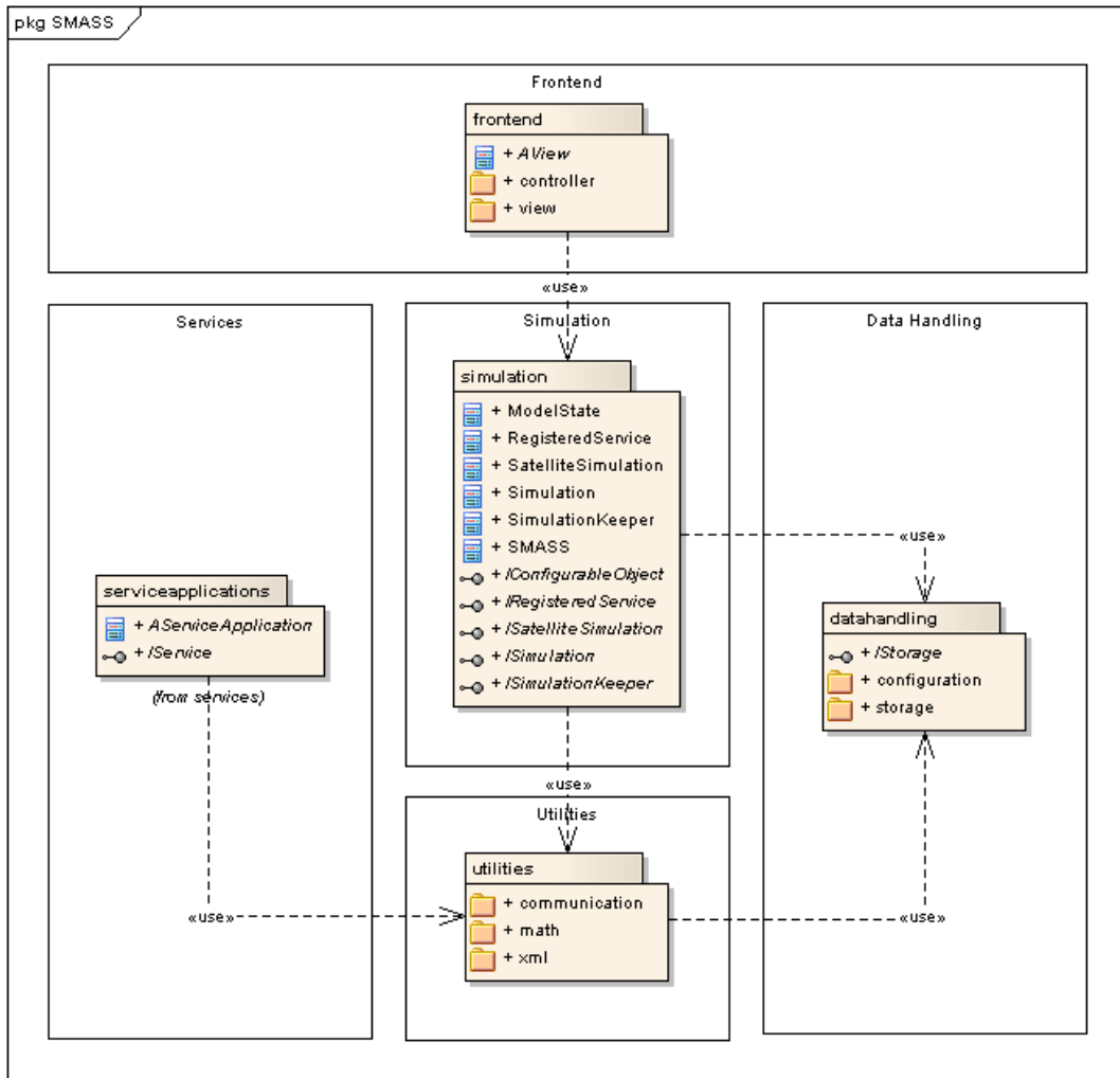
Fig. 3. Layers of new SMASS framework as UML package diagram
