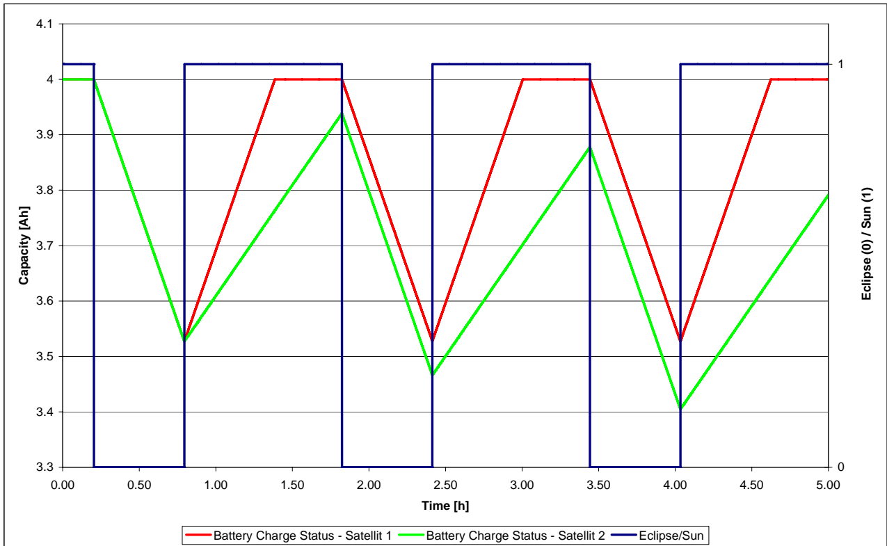
Fig. 6. Comparison of two different solar cell configurations on a satellite on the basis of accumulator charge statuses
