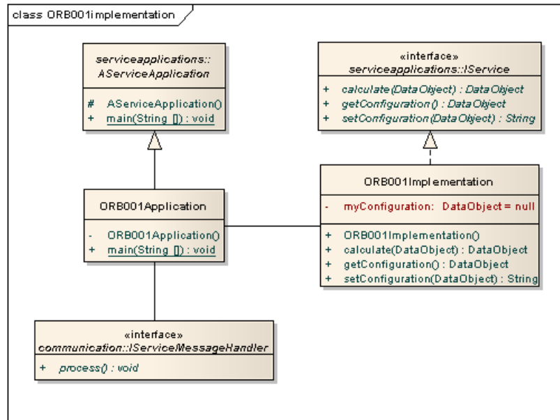
Fig. 5. Example of a service implementation for an orbit application as UML class diagram
