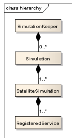
Fig. 4. Model hierarchy as UML class diagram
