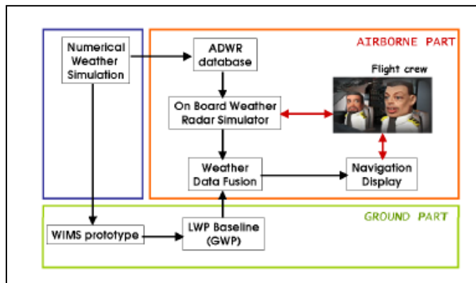
Figure 6. Weather data flow in the NLR Full Flight Simulator
