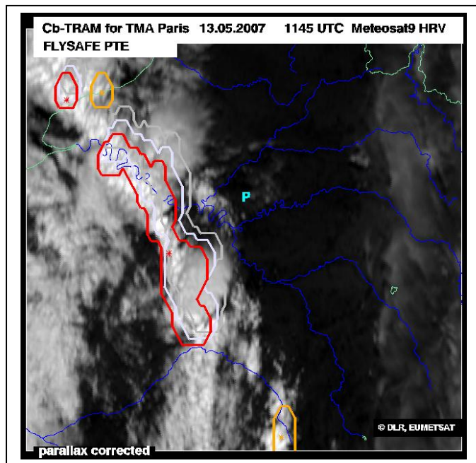
Figure 4. Cb top contours marked in colors of orange for “rapid development” and red for “mature thunderstorm”, overlaid on satellite imagery in the high resolution visible channel. Also marked are nowcast positions after 30 and 60 minutes in white and grey. TMA Paris on 13 May 2007, 1145 UTC
