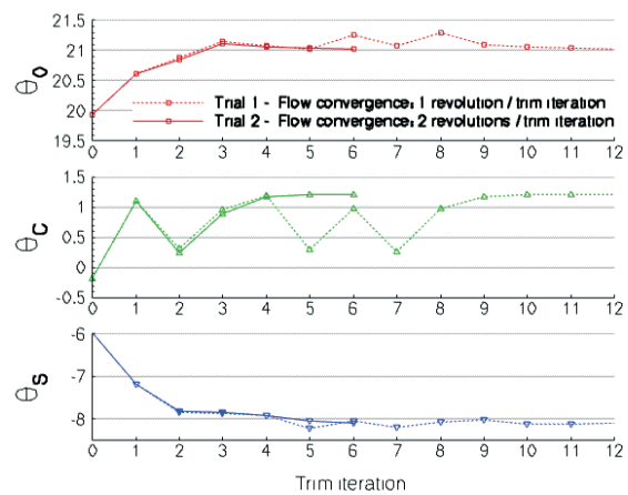
Figure 10: Free flight trim: Development of main rotor control angles \theta_0 (collective) and \theta_C, \theta_S (cyclic).
