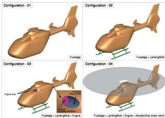
Figure 13: Increasing level of complexity in modelling the EC135 fuselage
