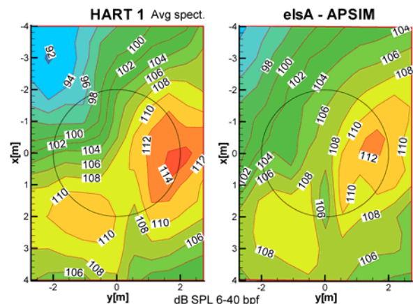
Figure 5: Measured and simulated noise levels for the HART1 Baseline Case.
