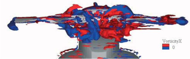
Figure 21: Vorticity distribution around the fixed complete rotor head (elsA computation).
