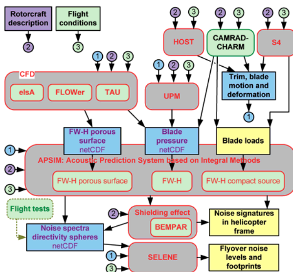
Figure 1: Possible tool (rounded boxes) linking into rotorcraft aeroacoustic prediction chains.
