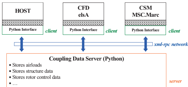
Figure 6: Schematic of the HOST-CFD-CSM coupling
