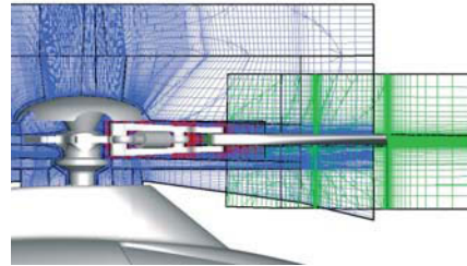
Figure 20: Chimera assembly example for the rotor hub computation.
