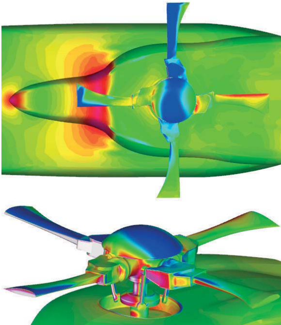
Figure 19: Pressure distribution on the EC145 engine cowling with rotating rotor head (model scale 1:73, v=40\text{m/s} , FLOWer solution).
