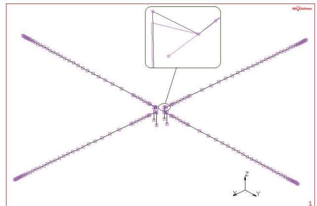
Figure 8: Finite-element modelling of the 7A rotor as beams with MSC-Marc
