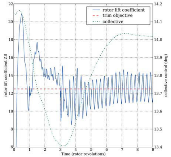
Figure 7: Evolution of collective pitch and lift coefficient for the 7A rotor at high-speed forward flight
