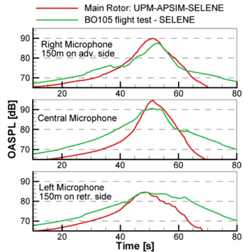
Figure 4: Fully simulated main rotor (red) and flight test interpolated (green) noise level time histories for a BO105 noise certification descent.
