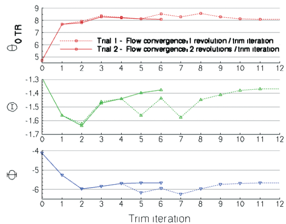
Figure 11: Free flight trim: Development of trim parameters \theta_{OTR} (tail rotor collective) and \Theta, \Phi (fuselage pitch and roll attitude).
