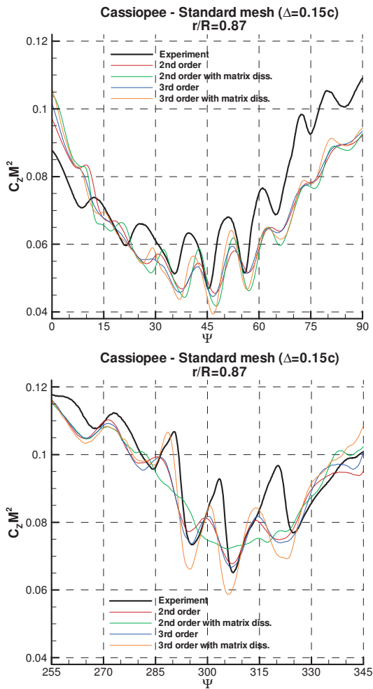
Figure 3: Computed BVI events on the advancing and the retreating blade sides
