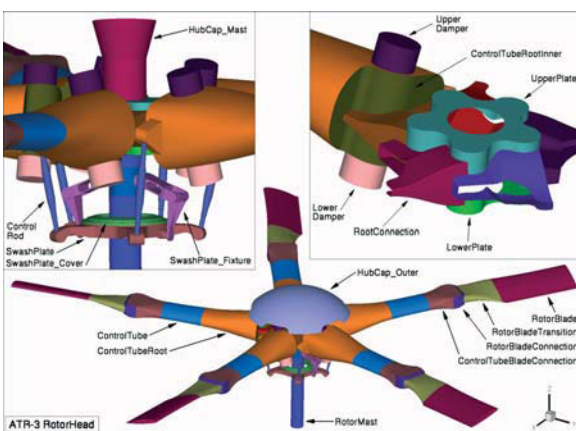
Figure 17: CAD geometry of detailed rotor head.
