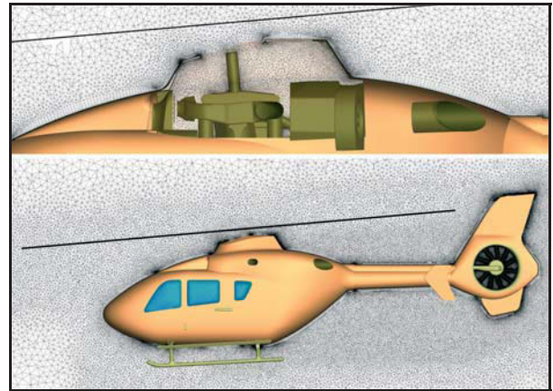
Figure 15: CENTAUR unstructured mesh about the EC135 helicopter including Fenestron® and upper deck with the rotors as actuator discs.
