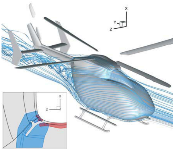
Figure 12: FLOWer simulation of EC145 helicopter, near-body streamlines on starboard half model. Insert: chimera blocks at skid attachment.
