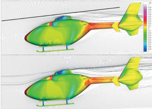
Figure 16: Pressure coefficient distribution on the EC135 surface and stream lines in the field with (top view) and without (bottom view) the main rotor modelled as actuator disc ( v=140kt , 5000ft, TAU solution).
