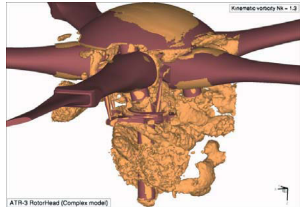
Figure 18: Instantaneous wake structure represented by constant kinematic vorticity surfaces on the detailed hub.
