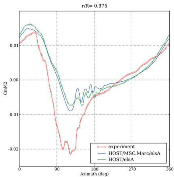
Figure 9: Comparison of HOST/MSC-Marc/elsA and HOST/elsA computed pitching moment evolution at r/R=0.975 for the 7A rotor
