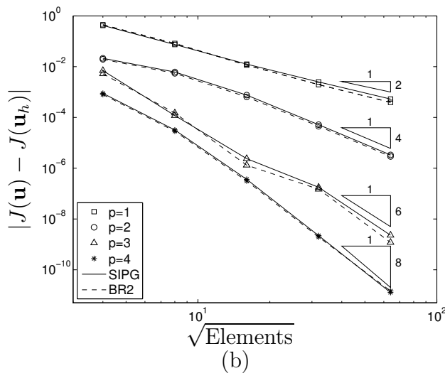
Fig. 2. Example 1. Comparison of the SIPG and BR2 methods when the error is measured in terms of: (a) L_2(\Omega) -norm; (b) Weighted mean-value functional J(\cdot) .
