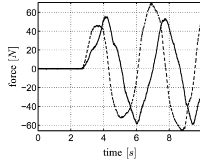
Fig. 7. Applied forces in x -direction (solid line) and y -direction (dashed line) in the first experiment.
