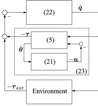
Fig. 3. System representation as an interconnection of passive subsystems.
