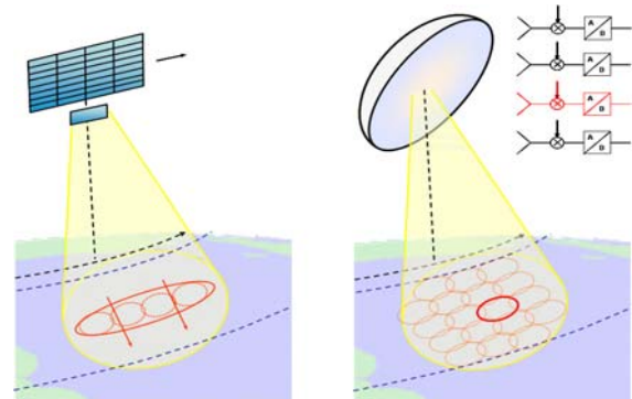
Fig. 2: Left: High-Resolution Wide-Swath (HRWS) SAR system employing direct radiating and receiving array antennas. Right: High-resolution wide-swath SAR employing a reflector antenna in combination with a digital feed array.
