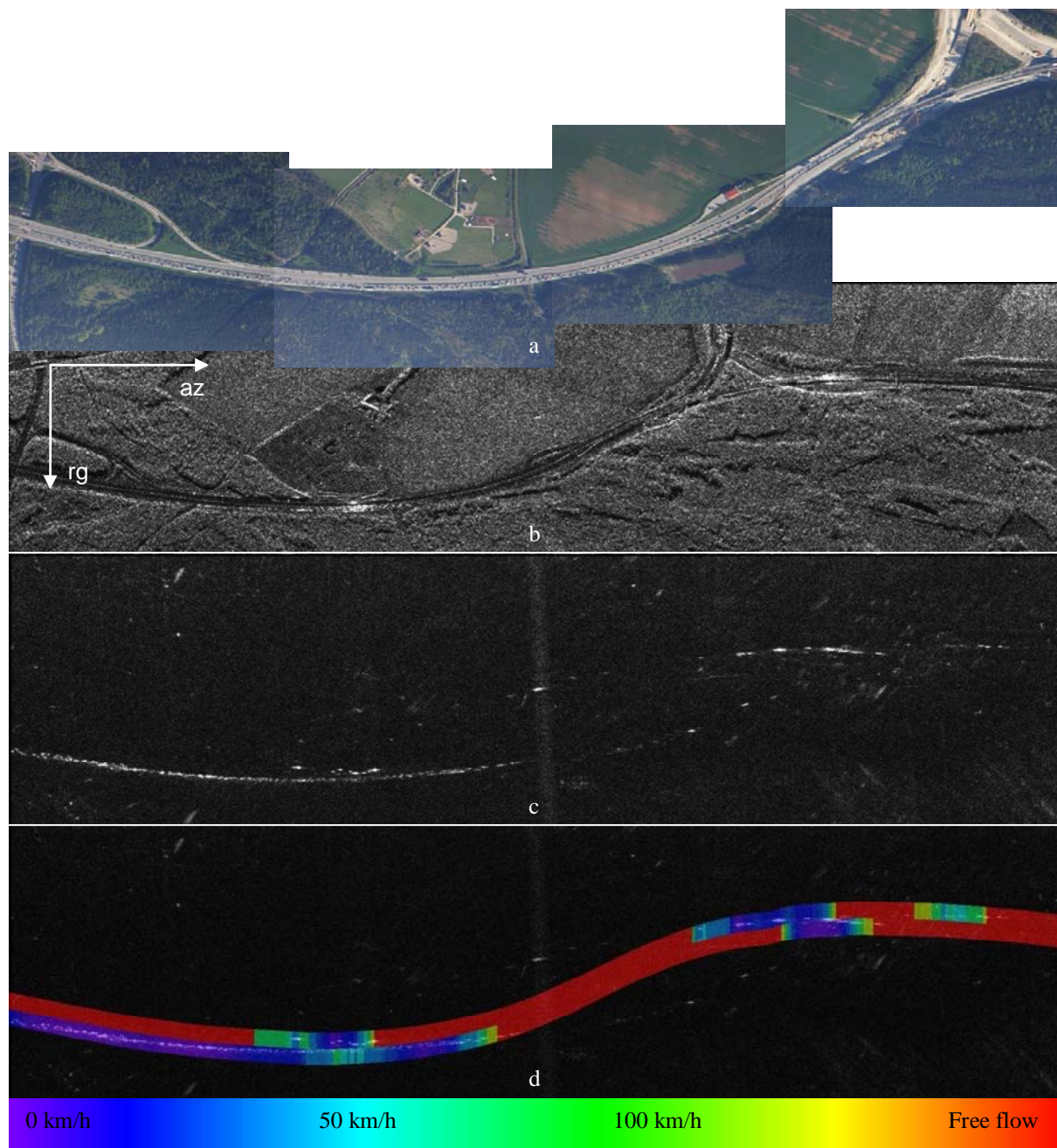
Fig. 1. The reference digital camera mosaic image of a part of highway between Germering and Munich, South Germany (a), E-SAR one channel amplitude image (b), DPCA image (c) and resultant velocity profile image with DPCA image in background (d).
