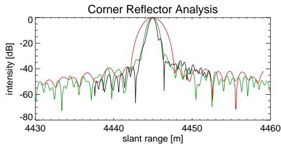
Figure 1: Performance check at a corner reflector. Achieved resolutions: 2.10m, 1.05m and 0.70m with 100 MHz, 200 MHz and 300 MHz Hamming weighted spectra (red,green,black). The used chirp replica for 300 MHz is not yet reliable.
