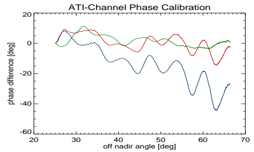
Figure 4: A priori phase differences in F-SAR ATI channels: red=VV1-VV2, green=VV1-VV3, blue=VV1-VV4, varying with range.
