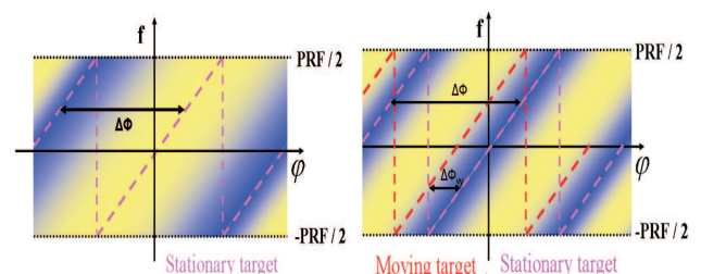
Figure 1: Filtering required for extracting the Nyquist sampled signal part (yellow: beam maximum, blue: beam minimum). Left: HRWS-SAR. Right: GMTI.
