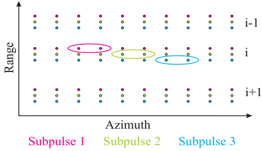
Figure 2: Clutter and its range/azimuth ambiguities for azimuth beamsteering on transmit with three subpulses and two azimuth ambiguities per subpulse due to azimuth subsampling. i - 1 denotes the ambiguities caused by the preceding, i + 1 the ambiguities by the subsequent pulse.
