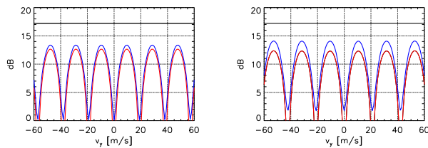
Figure 4: SINR after SAR compression for the medium out of three subpulses. Left: PRF = 1.22 kHz . Right: PRF = 1.35 kHz . (black: SNR in case of no interference, blue: SINR without azimuth beamsteering on transmit, red: with azimuth beamsteering on transmit.)
