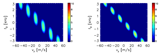
Figure 3: SINR after reconstruction and rearranging, but before SAR compression of moving target signals in five PRF bands ( SNR = 10 dB ). Left: Transmit antenna length: 7.2 m. Right: Transmit antenna length: 14.4 m.
