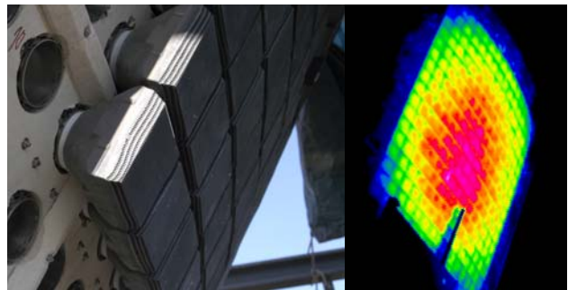
Fig. 5: Prototype receiver during assembly (left) and IR photograph during operation (right)
