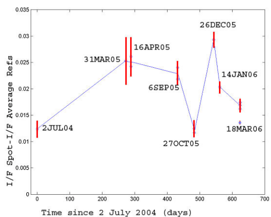
Fig. 2 Reflectance change at 2.02 \mu\text{m} Jul 04-Mar 06
