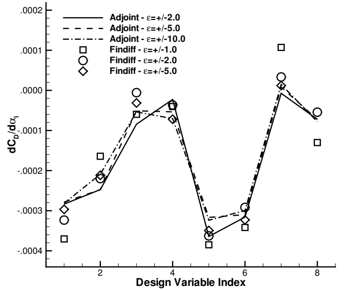
Fig. 6. Comparison of gradients evaluated with finite difference and adjoint for various step sizes.
