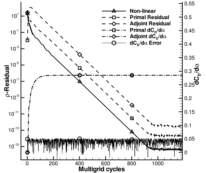
Fig. 1. Convergence of non-linear, primal and adjoint codes for an NACA0012 test case. Also shown are transients of dC_D/d\alpha .
