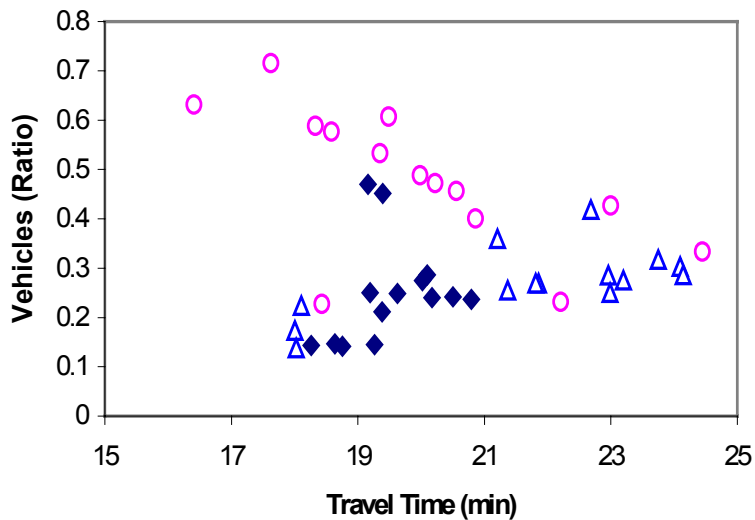
Figure 4: Correlation between the relative amount of vehicles on each route and the travel time on the same route. Symbols and correlation coefficients r : ◆: “Otto-Suhr-Allee” ( r = 0.23 ), ○: “Hansaplatz” ( r = -0.58 ), △: “Alt Moabit” ( r = 0.62 )
