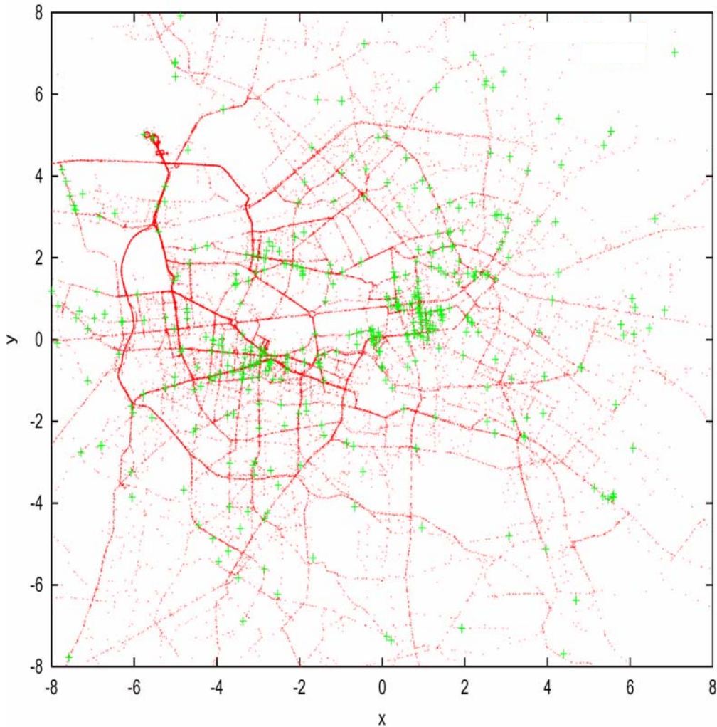
Figure 1: Distribution of taxi positions throughout the city of Berlin as obtained from GPS data collected in an historical data base. Crosses refer to destinations of occupied taxis started from Airport Berlin-Tegel.
