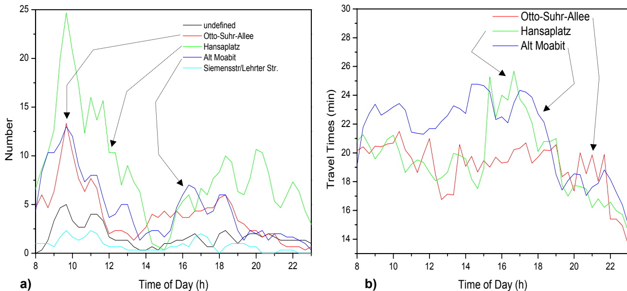
Figure 3: a) Numbers of occupied taxis using different routes between Airport Tegel and Friedrichstraße (20 min averages); b) Travel times needed for main routes (averaged)
