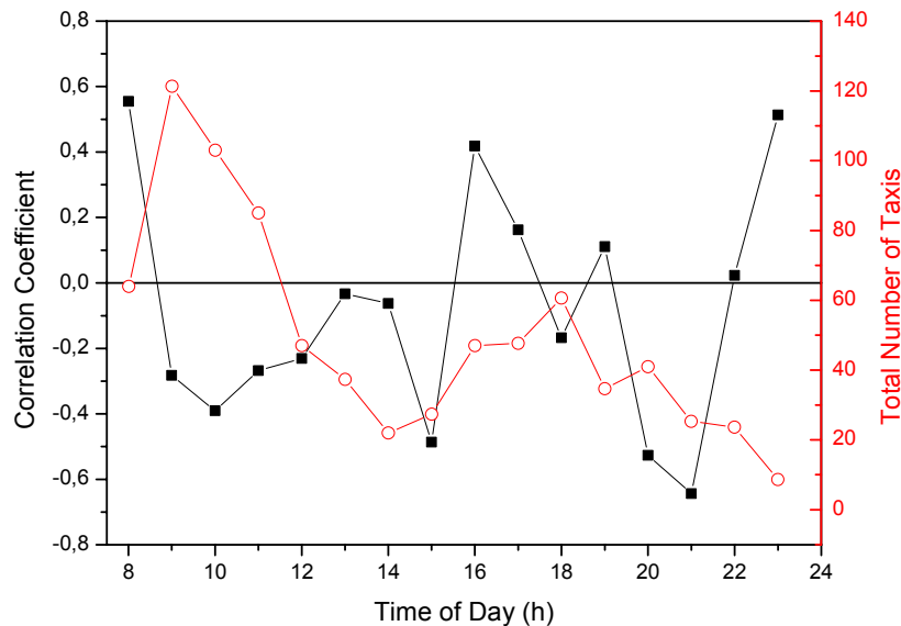
Figure 5: Correlation of taxi route choice with the route of shortest travel time. Left axes: correlation coefficient (■); right axes: total number of taxis per hour (○)
