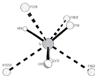
SiFHA 2 secondary (tetrel) bonding
