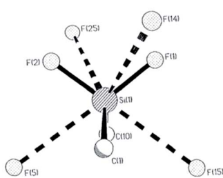
SiF 2 Ar 2 secondary (tetrel) bonding
