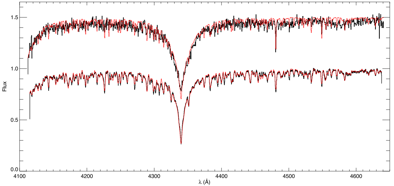
Figure 5. SME model fits (thin lines, red/grey) to the disentangled spectra (thick lines, black) of WASP 1628+10 A and WASP 1628+10 B (offset by +0.5 units).
