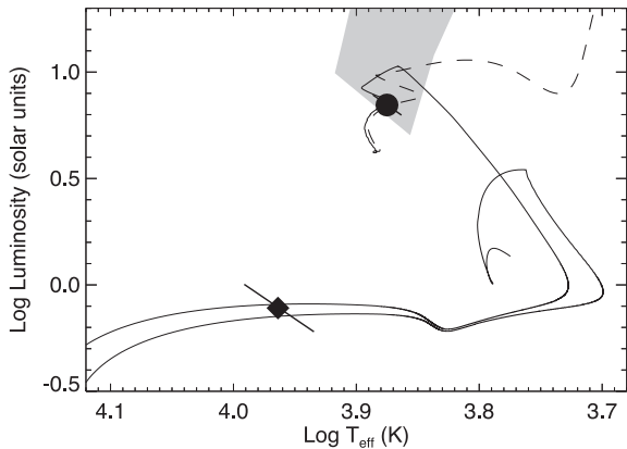
Figure 7. WASP 1628+10 A (circle) and WASP 1628+10 B (diamond) in the HRD. The dashed line is a model for a star with a mass of 1.36 M_{\odot} and metallicity Z = 0.006 . The solid line is a model for a star with an initial mass of 1.30 M_{\odot} in a binary system with a 0.8 M_{\odot} companion, orbital separation of 4.8 R_{\odot} and metallicity Z = 0.004 . The dot-dashed line is a model for a star with an initial mass of 1.0 M_{\odot} in a binary system with a 0.9 M_{\odot} companion, orbital separation of 4.8 R_{\odot} and metallicity Z = 0.008 . The instability strip for \delta Scuti-type pulsations with radial order k = 4 is indicated by light-grey shading (Dupret et al. 2004).
