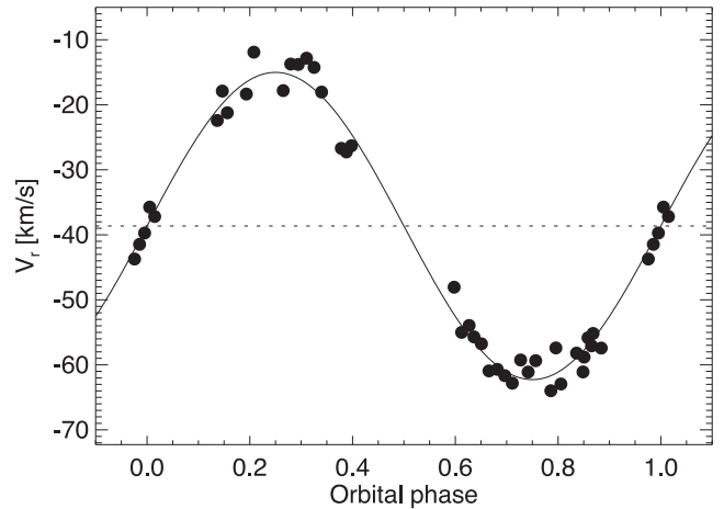
Figure 3. Radial velocities of WASP 1628+10 A, measured using cross-correlation against a synthetic template spectrum generated by SME for the parameters T_{\text{eff}} = 7500 \text{ K} , \log g = 4.2 , V_{\text{rot}} \sin i = 105 \text{ km s}^{-1} . The solid line is a circular orbit with the parameters K_A = 23 \text{ km s}^{-1} and the dotted line indicates the mean radial velocity \gamma = -39 \text{ km s}^{-1} .
