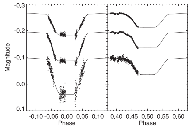
Figure 2. From bottom-to-top: ULTRACAM u' , g' and r' light curves of the primary and secondary eclipses of WASP 1628+10 (points) with our least-squares fits to these data (lines). Note that the model fits shown do not include the modulation of the signal due to pulsations.
