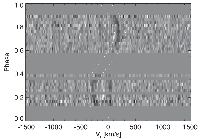
Figure 4. Grey-scale plot showing spectra of WASP 1628+10 after subtraction of a synthetic spectrum for WASP 1628+10 A. The sinusoidal signal highlighted with dotted lines is the \text{Mg II } 4481 \text{ \AA} line from WASP 1628+10 B. The absorption and emission features near 0 \text{ km s}^{-1} are residuals from the spectral subtraction due to line profile variations in WASP 1628+10 A.
