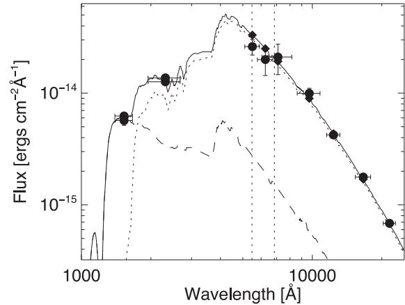
Figure 6. Model fit to the observed flux distribution of WASP 1628+10 used to estimate the effective temperatures of WASP 1628+10 B. The observed fluxes are shown as circles with error bars. The predicted contributions of each star to the observed fluxes are shown as dotted or dashed lines and their sum is shown as a solid line. The models have been smoothed slightly for clarity in these plots. Diamonds show the result of integrating the total model flux over the band width indicated by horizontal error bars on the observed fluxes. The assumed band width of the r' filter is indicated with vertical dotted lines. The model for WASP 1628+10 A has T_{\text{eff}} = 7400 K [\text{Fe}/\text{H}] = -0.5 and \log g = 4.25 . The model for WASP 1628+10 B has T_{\text{eff}} = 9800 K, [\text{Fe}/\text{H}] = -0.5 and \log g = 4.5 . A reddening of E(B - V) = 0.056 has been assumed.
