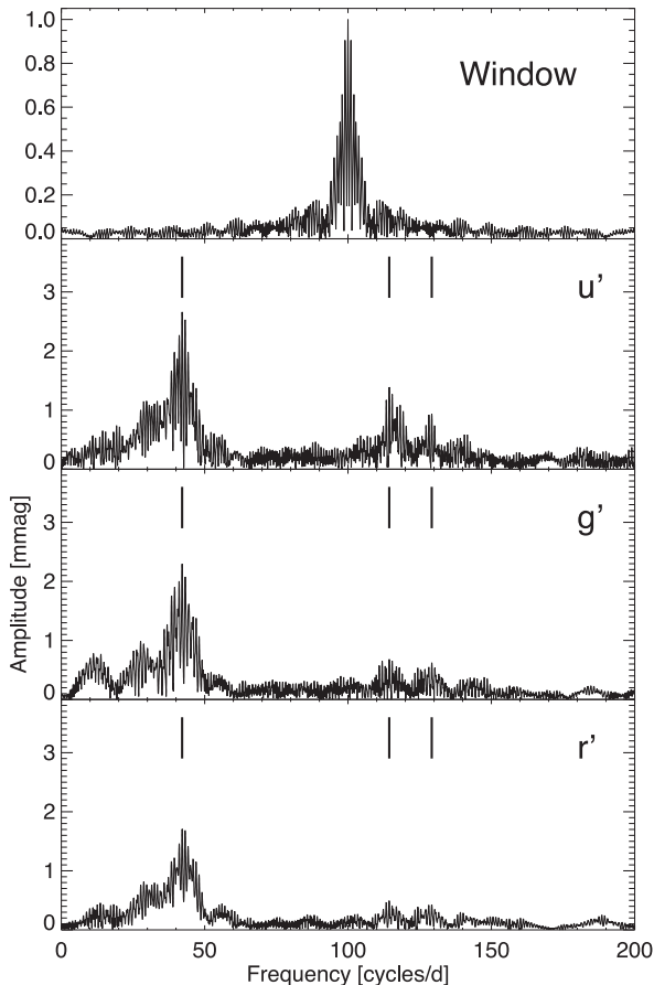
Figure 1. Periodograms of the out-of-eclipse ULTRACAM data of WASP 1628+10. The three frequencies detected in all three channels are indicated.
