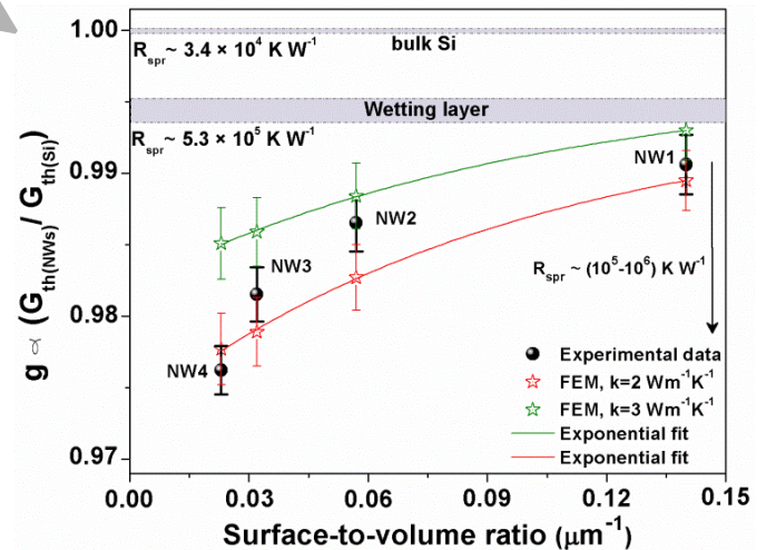
Figure 8. Plot of the experimental thermal ratio ( g ) (black spheres) and the ratio obtained from the FEM simulations ( g_{FEM} ) (red and green stars) versus the surface to volume ratio of the \text{Si}_{1-x}\text{Ge}_x NWs.
