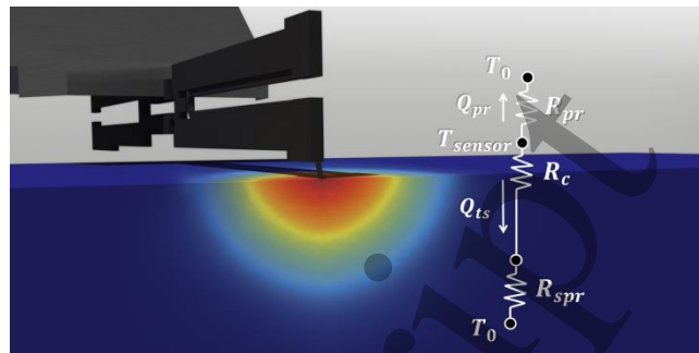
Figure 7. Schematic of the nanoscopic tip-sample contact and the equivalent thermal resistance circuit.
