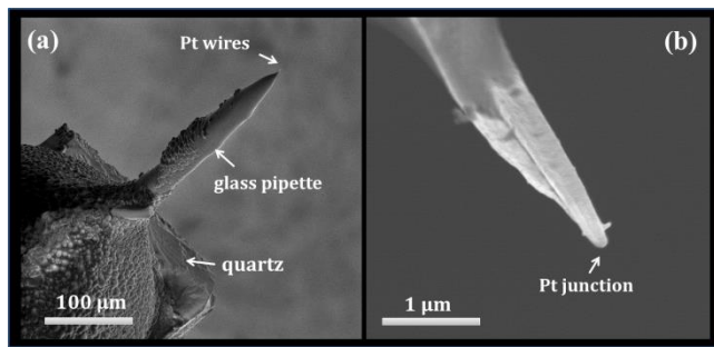
Figure 5. SEM images of (a) the SThM probe with the integrated Pt resistive elements and (b) the nanometer-scale junction in the Pt wires.
