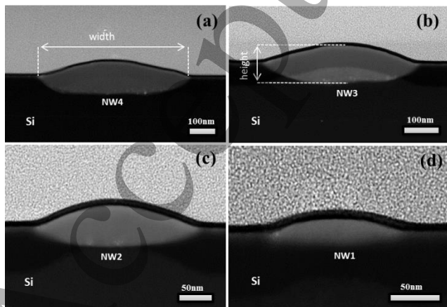
Figure 2. (a)-(d) Cross-section TEM images of the four
