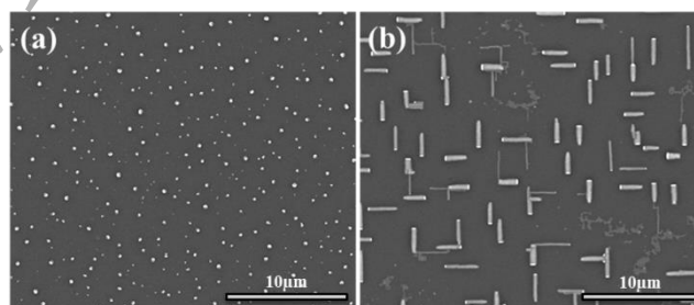
Figure 1. SEM images of (a) the AuSi seeds after 5 minutes annealing of the Au and Si layers at 800 °C and (b) the in plane epitaxial \text{Si}_{1-x}\text{Ge}_x alloy NWs after the Ge deposition by MBE.
