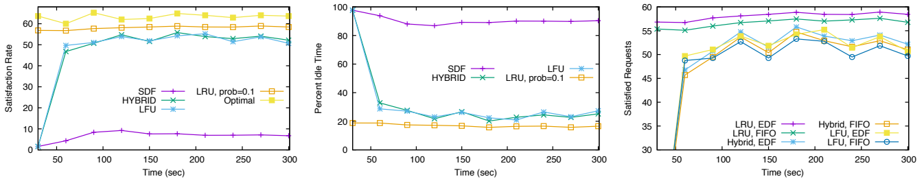
Fig. 7: Performance of strategies using trace-based workload.
