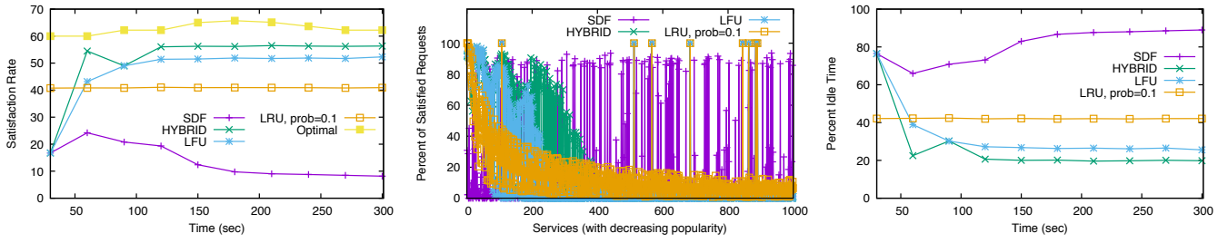
Fig. 3: Performance of strategies with service popularity uncorrelated with deadlines.
