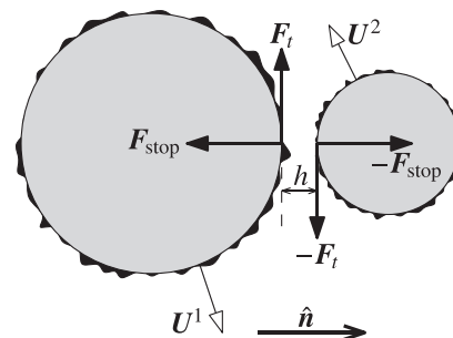
FIG. 4. The normal contact force, \mathbf{F}_{\text{stop}} , and tangential friction force, \mathbf{F}_t , oppose the motion of the approaching particles. These forces are added to any existing forces – hydrodynamic, gravity, etc. – already acting on the particles.
