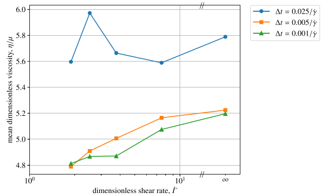
FIG. 11. The effect of varying the timestep \Delta t . Plot of the mean steady viscosity with model parameters \nu = 0.3 , h = 0.01a , and a periodic box containing 90 spheres at an area fraction of 69.3%. A timestep \Delta t = 0.025\dot{\gamma}^{-1} is too large to make meaningful predictions; but the marginal gain in accuracy by reducing from \Delta t = 0.005\dot{\gamma}^{-1} to \Delta t = 0.001\dot{\gamma}^{-1} does not merit the extra computational effort involved.
