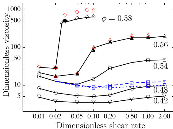
FIG. 2. Continuous and discontinuous shear thickening is observed here at varying volume concentrations ( \phi ). Graph reproduced with permission from Seto et al. , “Discontinuous shear thickening of frictional hard-sphere suspensions,” Phys. Rev. Lett. 111 , 218301 (2013). Copyright 2013 American Physical Society.
