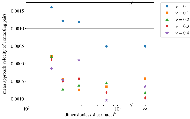
FIG. 6. Mean approach velocity (across all contacting pairs) for simulations with different values of \nu and \dot{\Gamma} . All values are at most of magnitude 10^{-3} , which is rather small, so we can conclude that our normal forces are indeed a good approximation to those which exactly halt particle approach. There is no systematic dependence on either friction coefficient or shear rate; these values are just small-magnitude noise.
