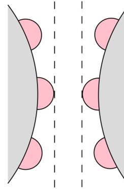
FIG. 3. Schematic of a roughness model. The pink bumps represent sparse surface asperities, which prevent the particles from approaching closer than a nominal roughness height while leaving hydrodynamic forces unchanged.
