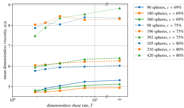
FIG. 12. The effect of system size. Model parameters \nu = 0.3 , h = 0.01a , and we are using the Ball–Melrose approximation to save computation time. At the highest concentration, box size effects are important; at c = 69\% 90 particles will suffice and at c = 75\% we use 98 particles.
