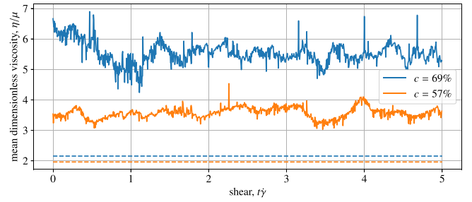
FIG. 10. Dimensionless viscosity under shear, measured over five shear units. Here the friction coefficient is \nu = 0.3 , roughness height h = 0.01a , timestep \Delta t = 5 \times 10^{-3}\dot{\gamma}^{-1} and the dimensionless shear rate is \dot{\Gamma} = 6\pi . Each periodic box contains 90 identical spheres. The dashed lines represent the dilute viscosity limit for each concentration, 1 + 5c/3 .
