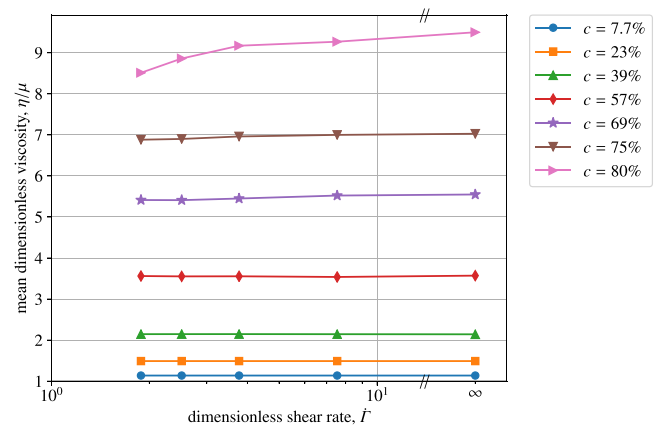
FIG. 14. Dependence of the dimensionless viscosity on dimensionless shear rate at different values of the area fraction c . At concentrations up to 69\% we use full Stokesian Dynamics with 90 particles; at 75\% we use 98 particles; and at the highest concentration we use the Ball–Melrose approximation to allow us to use more particles. The model parameters are h = 0.01a and \nu = 0.3 .
