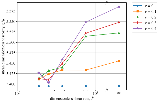
FIG. 15. Plot of dimensionless viscosity against dimensionless shear rate for a system with area fraction c = 69.3\% , h = 0.01a and a range of values of the friction coefficient \nu . There are 90 particles in the periodic cell and we are using full Stokesian Dynamics.
