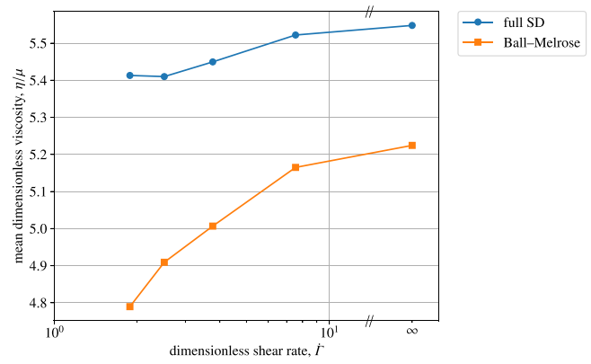
FIG. 13. Comparison of the viscosity calculated by full Stokesian Dynamics with the Ball–Melrose approximation. Simulations of 90 spheres at an area fraction c = 69.3\% , using \nu = 0.3 and h = 0.01a .
