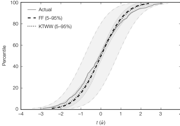
FIGURE 2 CDFs: Net Returns t(\hat{\alpha})
