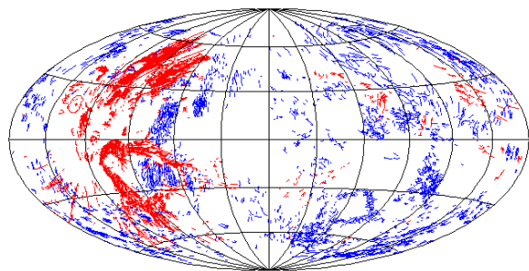
Fig. 1: Surface Faults on Mars. Red: normal faults, Blue: thrust faults. Map in Hammer's projection, centered to 0°N0°E.
