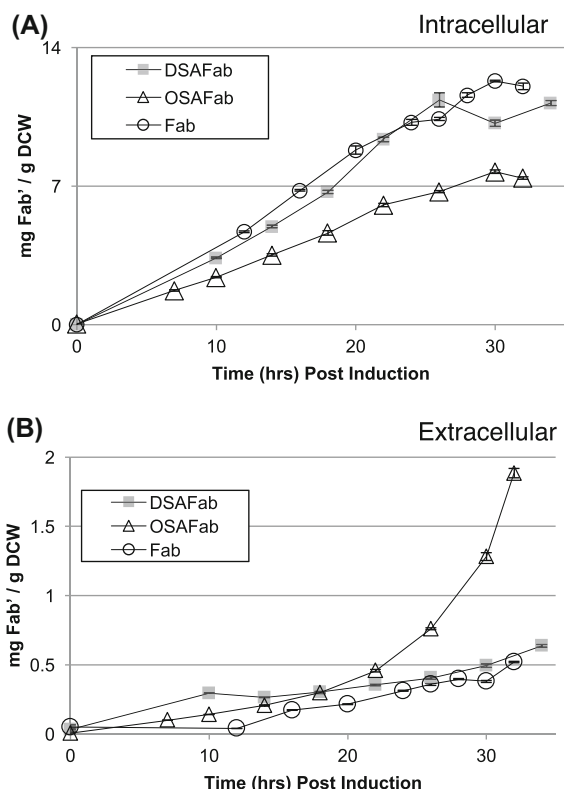
Fig. 3 Fab' fragment production and leakage. a Specific, post-induction, intracellular Fab' levels measured for the Fab, OSAFab and DSAFab strains during bioreactor cultivation. b Specific, post-induction, Fab' levels measured in the growth medium for Fab, OSAFab and DSAFab strains during bioreactor cultivation
