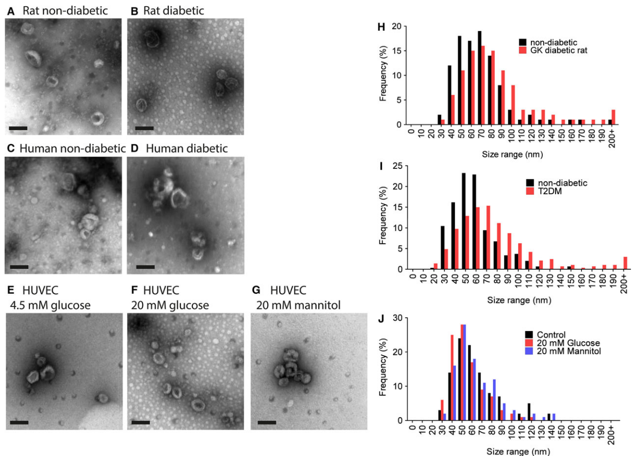
Fig. 2 Transmission electron microscopy (TEM) of exosomes isolated from the blood of rats (A and B), human patients (C and D) or from cultured HUVECs under the cultured conditions indicated (E–G). Bar = 100 nm. (H–J) Size distribution diameters from TEM images of vesicles from rats (H) ( N = 399 and 505 ), humans (I) ( N = 297 and 284 ) and HUVECs (J) ( N = 59 , 294 and 131 ). No significant difference was found when distributions were compared by Mann–Whitney U -test or Kruskal–Wallis test for 2 or 3 groups, respectively.
