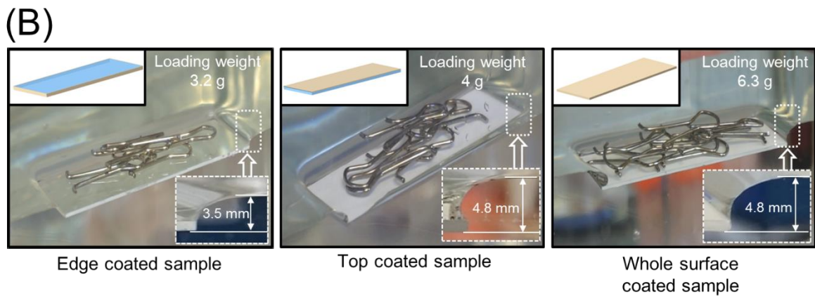
Figure 4. (a) Buoyancy test of control, bottom-, edge-, top-, and whole surface-coated glass microscope slides, and (b) loading capacity of edge-, top- and whole surface-coated samples.
