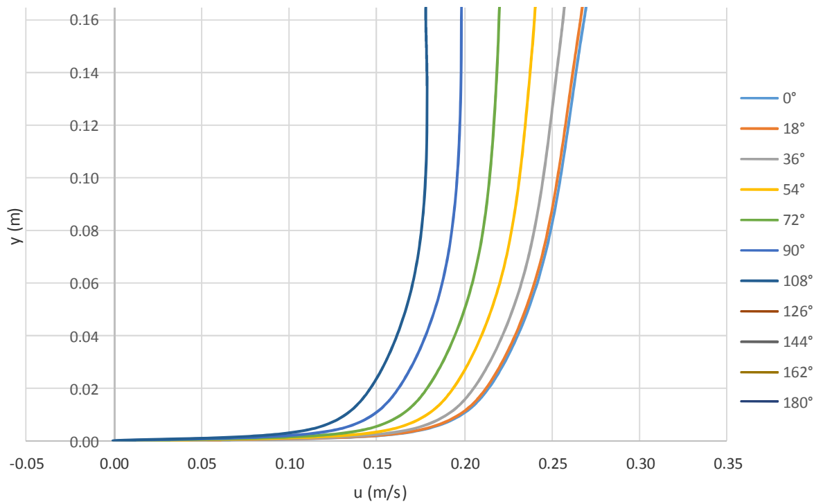
Figure 6. – Velocity profiles at 18° interval within full depth, WCA1 (CFD results)
