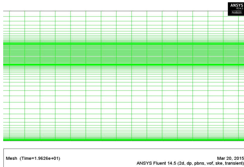
Figure 1. – Model grid. Part of the mesh, combined wave-current flow
