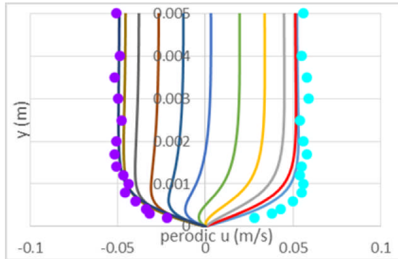
Figure 3. – Periodic velocities in the bottom boundary layer, WCA1 (CFD results presented as lines, experimental data presented in dots).
