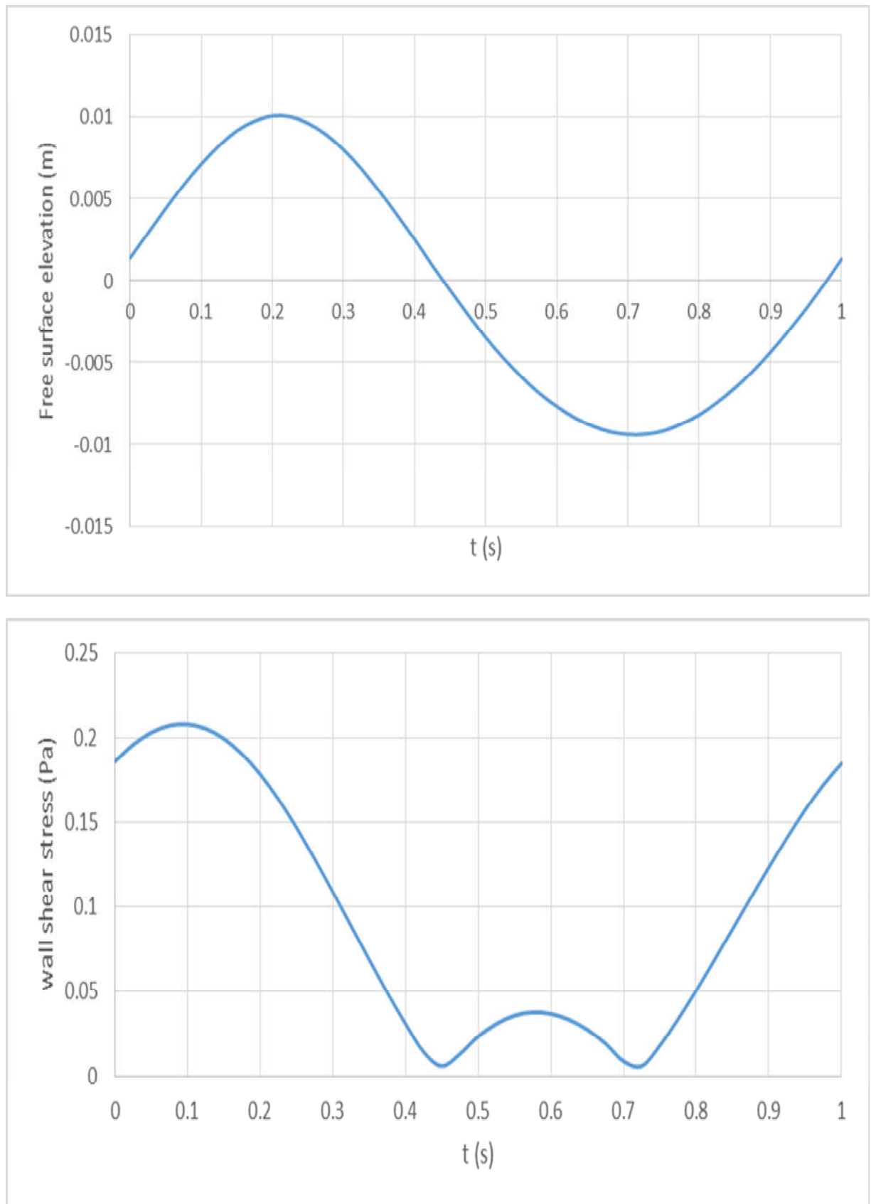
Figure 7. – Time series of (a). free surface elevation and (b). bed shear stress, waves propagating with a current, given d=200\text{mm} , T=1\text{s} , H=0.02\text{m} , U=0.185\text{m/s} .
