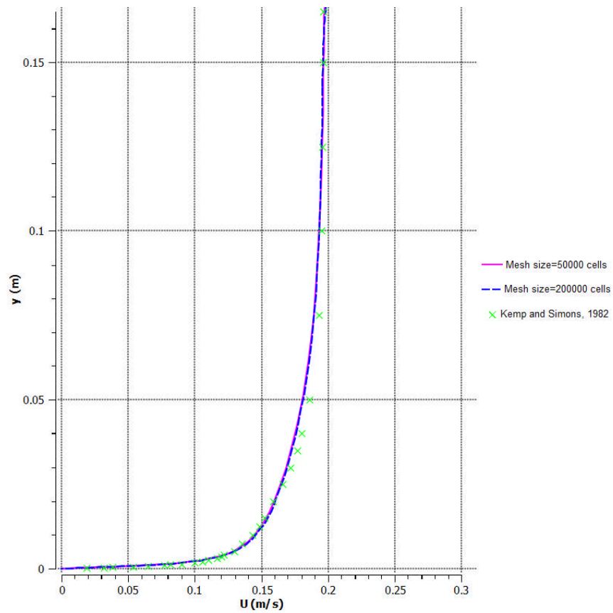
Figure 5. – Convergence of numerical results for mean horizontal velocity profile for the case WCA1. Time step = 0.001s, mesh size = 50k and 200k cells.
