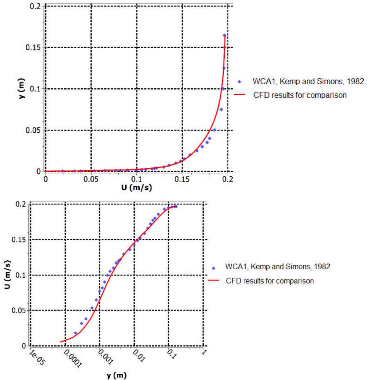
Figure 2. – Mean horizontal velocity profile for waves propagating with a current, given d=200\text{mm} , T=1\text{s} , H=0.02\text{m} , U=0.185\text{m/s} , (a) linear scale; (b) semi-logarithmic scale.
