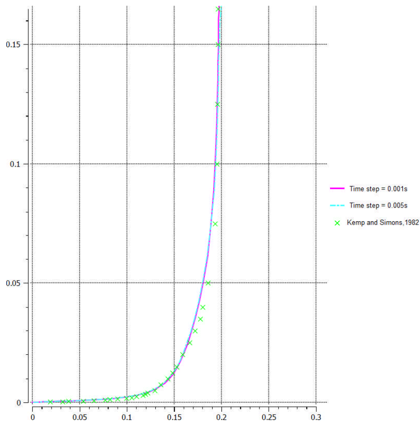
Figure 4. – Convergence of numerical results for mean horizontal velocity profile for the case WCA1. Meshes with 50k cells, and two time steps = 0.005s and 0.001s.
