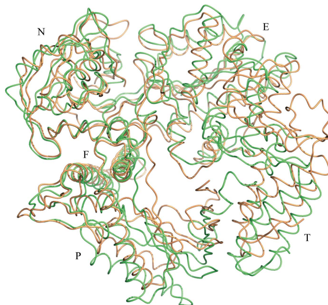
Figure 3 A superposition of Pc -polymerase with Pfu DNA polymerase. The structures are coloured cream for Pc -polymerase and green for Pfu DNA polymerase, with the N-terminal, exonuclease, palm, fingers and thumb domains labelled N, E, P, F and T, respectively. The thumb domain undergoes the greatest movement upon binding to the DNA substrate, moving away from the catalytic centre.
