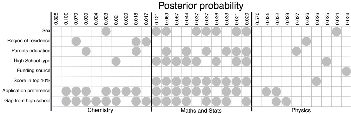
Figure 5: BMA posterior inference. Top 10 models according to posterior probability, for each degree programme. Gray circles indicate covariate inclusion.
