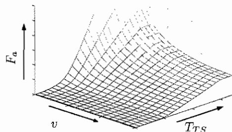
Fig. 1. Static assist characteristics of an exemplary EPS system.
