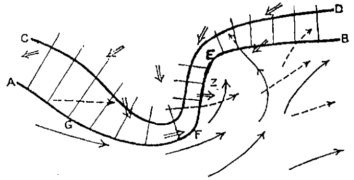
FIG. 14. Form and position of the separation surface between cold and warm air in a cold-tongue region. Full single arrows: warm airflow at the surface; dashed arrows: warm airflow aloft; double arrows: cold surface airflow (Exner 1920, Fig. 6).
