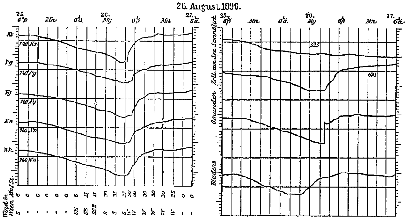
FIG. 8. Surface pressure traces for the period 25 August, 6 p.m., until 27 August 1896, 6 a.m., for a mesoscale network of stations around Vienna (left) and other stations in the west of Austria (right). Vertical lines every two hours; Mn: midnight; Mg: noon; tick marks every 1 mm Hg (= 1.33 hPa); horizontal lines designate reference pressure of 740 mm Hg, except for Zell am See (695 mm Hg) and Sonnblick (525 mm Hg). Station codes: Ks - Krems, Pg - Bratislava, Fg - Feldsberg, Nn - Neunkirchen, Wn - Vienna. Wind speed (km h -1 ) and direction for Vienna are given every 2 hours under the left diagram (Murgules 1897, Fig. 5).
