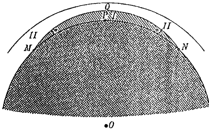
FIG. 13. Polar cap of a cold air mass (I) underneath a warm air mass (II). O , center of the earth; P , north pole; M O P N , span of the solid earth (Exner 1917, Fig. 58).
