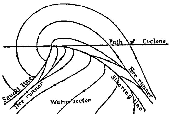
FIG. 1. First appearance of the Norwegian cyclone model and its flow structure. The components are an asymmetric cyclone moving from left to right, a sector of warm air in the south, and two separation lines ahead of and behind the warm sector (JB19, Fig. 1).
