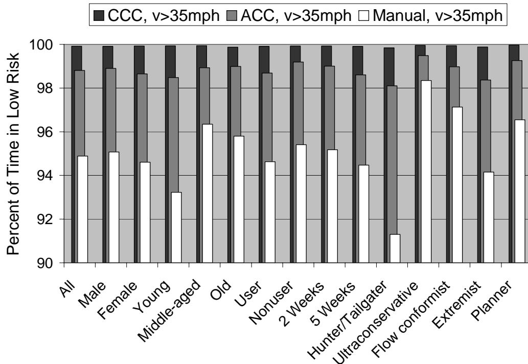
Figure 4: Comparison of the percent of time in the low risk state in every driving mode for different driver groups.
