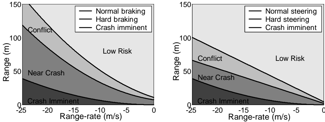
Figure 1: Boundaries of the performance map in the range vs. range-rate plane. Left: The state boundaries describing the last-second braking response. Right: The state boundaries of the last-second steering response.
