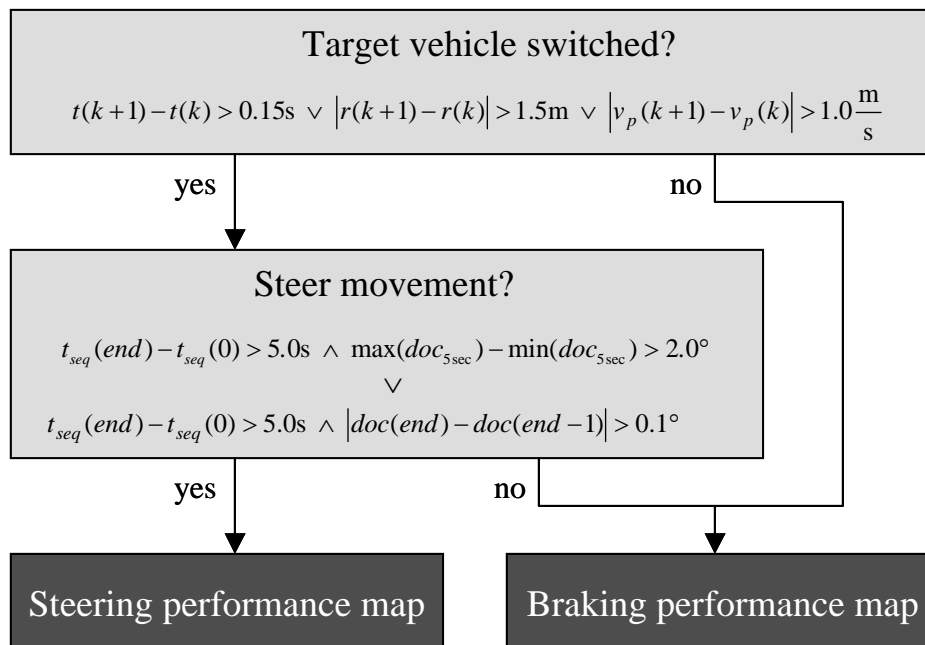
Figure 2: Flowchart of the algorithm for identifying steering movements prior to a target vehicle switch.
