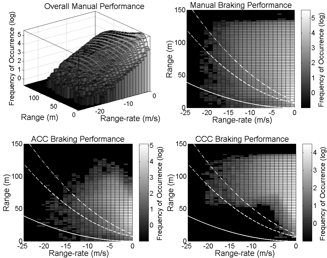
Figure 5: Frequency of occurrence (log) of data records in a rasterized range vs. range-rate plane. Top left: The frequency of occurrence of the overall manual driving in a three-dimensional depiction. Top right: Top view of the manual braking performance. Down left: Top view of the ACC braking performance. Down right: Top view of the CCC braking performance. The lines in all three top view plots denote the transition boundaries between the different driving states, respectively.
