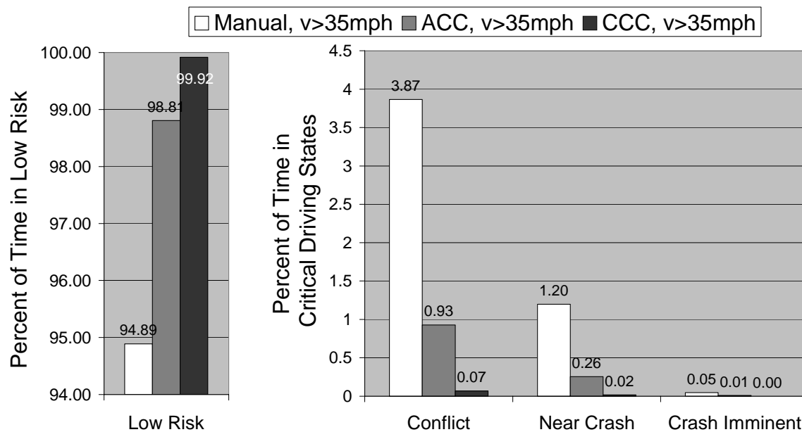
Figure 3: Comparison of the percent of time in the different driving states in every driving mode for all drivers.
