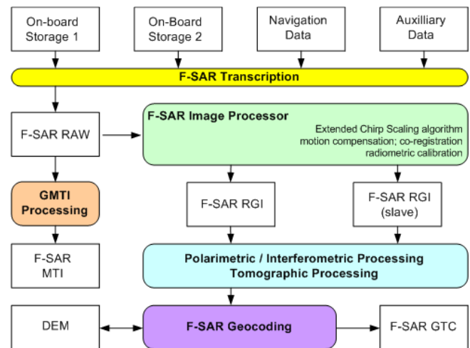
Figure 6 F-SAR processor block diagram.
