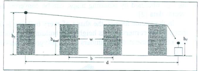
Fig. 6: Basic approach of the Walfisch-Ikegami and COST-231 model
