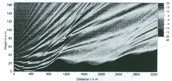
Fig. 7: Computation of the path loss in a vertical plane with the parabolic equation method for DAB broadcasting (frequency 1500 MHz)
