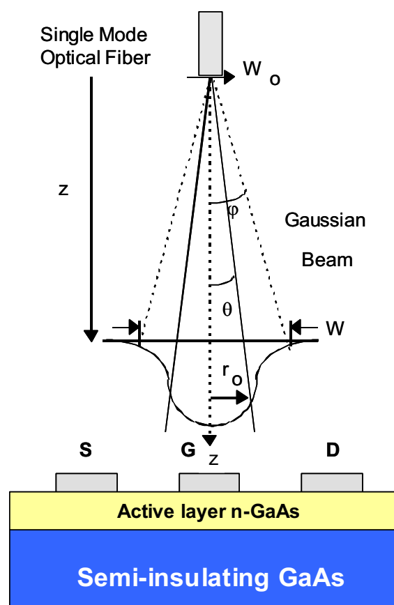
Fig. 1. Optical measurement set-up.
