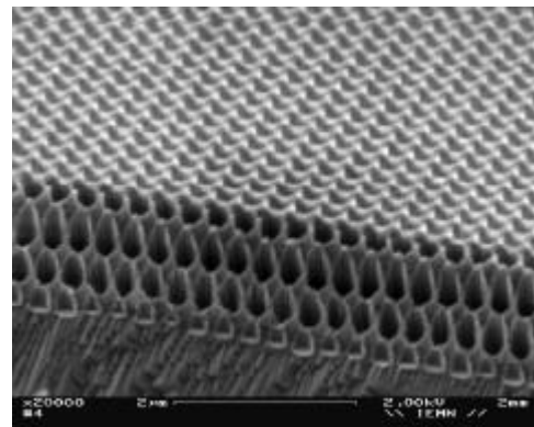
Fig.3b Array of nanoscaled tips on GaAs(Courtesy of A. Vanoverschelde, IEMN)
