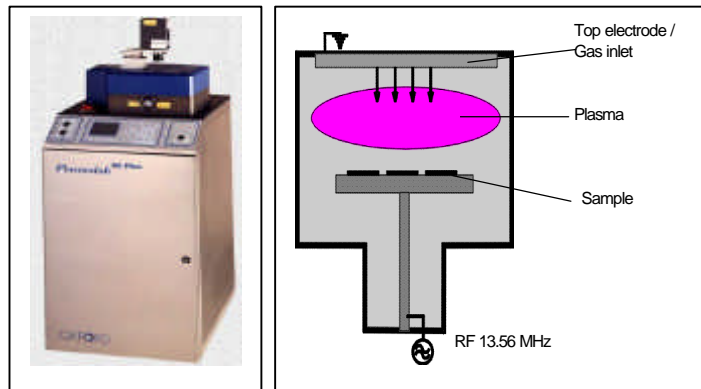
Figure 1: (a) RIE machine (b) Cross sectional view.
