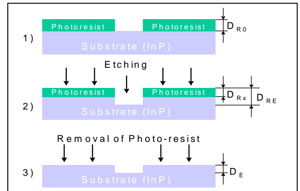
Figure 2: Etching process of InP
