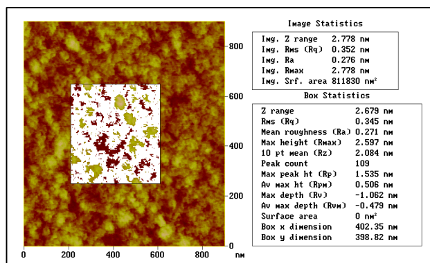
Figure 3: Determination of surface roughness using AFM
