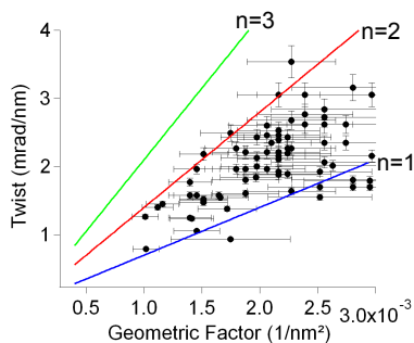
FIG. 2. NW twist rate as a function of the inverse of the cross sectional area. The blue, red and green lines represent the twist rate for screw dislocations with |b| = 0.68 nm ( n = 1 ), |b| = 1.36 nm ( n = 2 ) and |b| = 2.04 nm ( n = 3 ), respectively. Even considering the uncertainties on the cross sectional area, the twist data is not consistent with any of the suggested burgers vectors.
