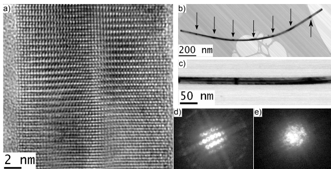
FIG. 1. a) HRTEM image showing a discontinuity of the atomic planes at the center of the NW. The contrast changes along the NW growth direction. b) BF STEM image of a NW showing a periodic set of dark bands (marked by arrows). c) BF STEM image of the region from which the CBED movie M1 in the Supplemental Material has been made. d) and e) Experimental CBED patterns from the two primary bands on c).
