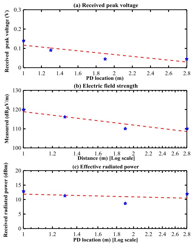
Figure 16. (a) Peak voltage, (b) Electric field strength, and (c) ERP as a function of antenna distance from the emulator (acrylic tube internal emulator without oil filling).
