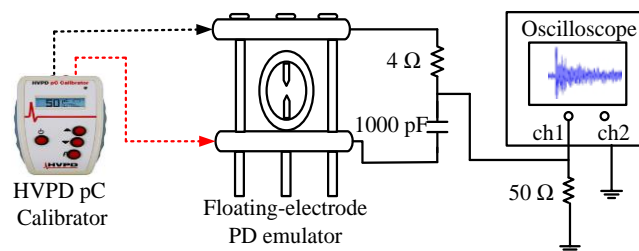
Figure 13. Measurement circuit for emulator calibration.
