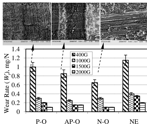
Fig.1 Wear rate, associated with SEM, of the KFRC at different orientations
