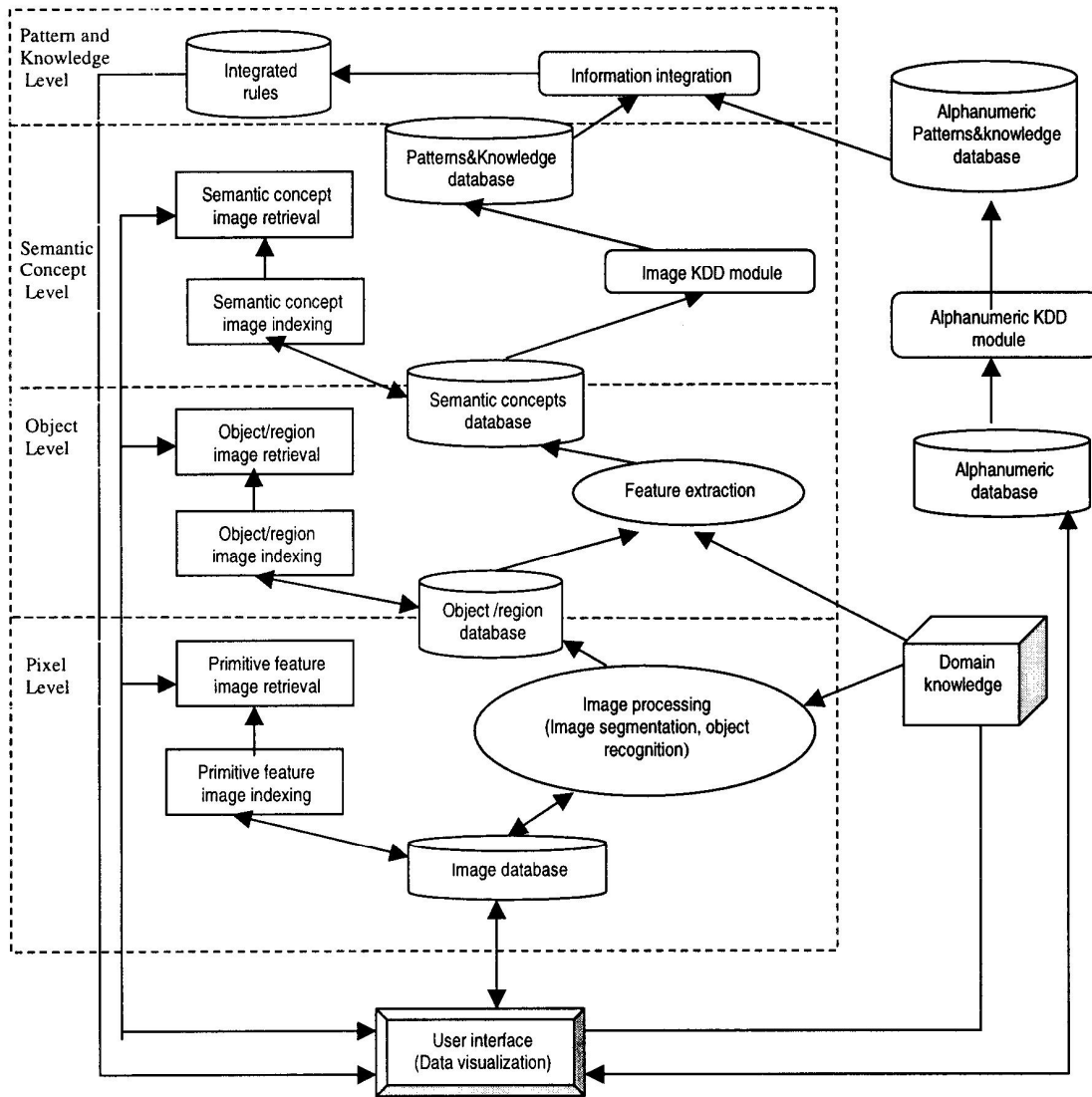
Figure 2: An information-driven image mining framework
