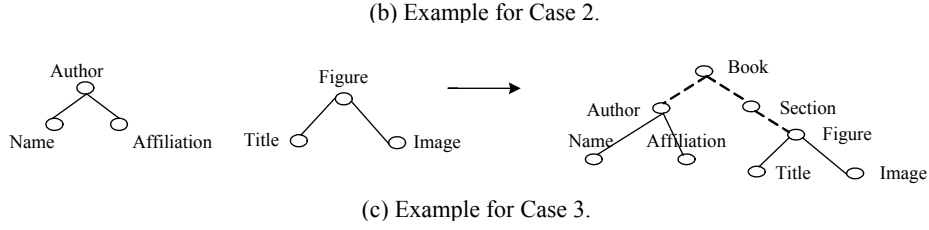
Fig. 6 (a) – (c). Examples of FreqQPT merging.
