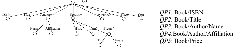
Fig. 1. Global DTD Tree of multiple XML documents. Fig. 2. QPs of the XQuery sample.
