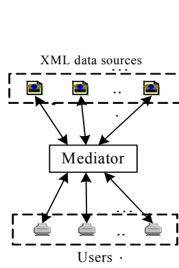
Fig. 7. Query processing without data warehouse
