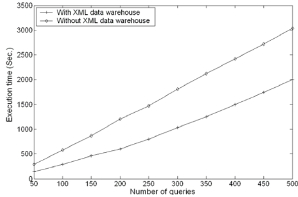
Fig. 10. Comparative study on query answering time
