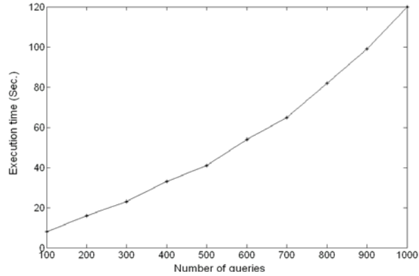
Fig. 9. Efficiency of constructing the data warehouse schema under varying number of queries
