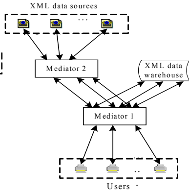
Fig. 8. Query processing with data warehouse
