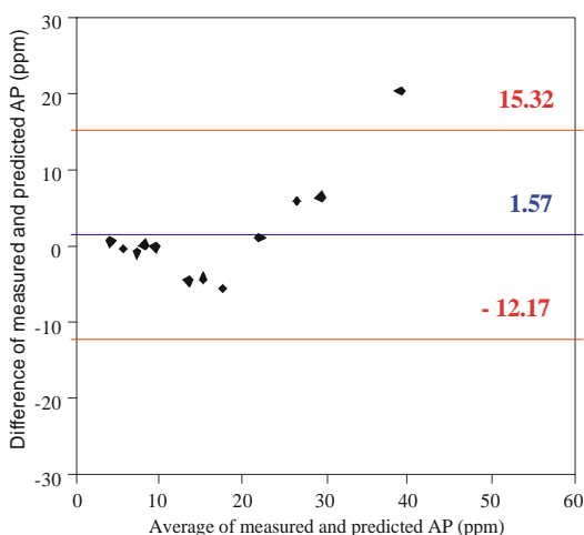
Fig. 2: Bland-Altman plot for the comparison of measured AP and predicted AP using the soil AP pedotransfer function; the outer lines indicate the 95% limits of agreement (-12.17, 15.32) and the center line shows the average difference (1.57)
