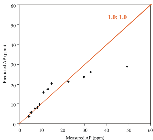
Fig. 1: Measured and predicted AP using the soil AP pedotransfer function with the line of equality (1.0: 1.0)
