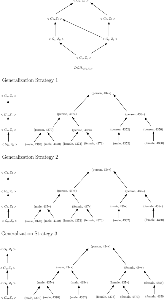
Figure 2: Hierarchy DGH_{\langle G_0, Z_0 \rangle} and corresponding domain and value generalization strategies
