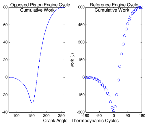
Figure 2. Matlab model plot of comparison between thermodynamic cycle work of the opposed piston engine and a reference engine.
