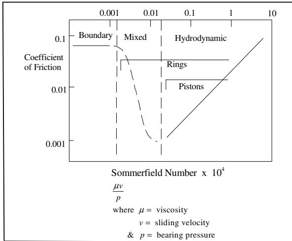
Figure 3. Engine lubrication regimes defined in the Stribeck diagram. The diagram reflects the general nature of engine friction. Only the piston skirts operate in full hydrodynamic conditions in conventional engines referred to here. Adapted from Stone [12]
