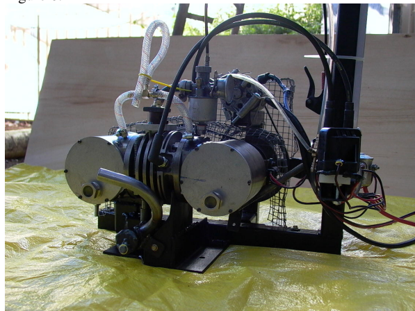
Figure 6. Prototype engine and frame during early attempts to start the engine
