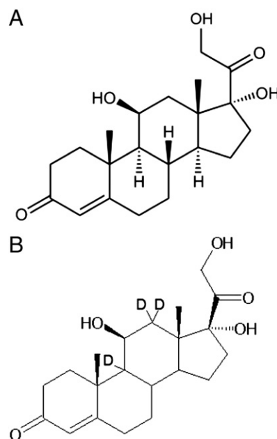
Fig. 1. Molecular structure of A) cortisol and B) d 3 -cortisol.
