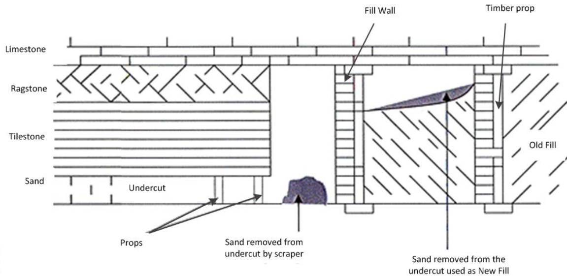
Figure 13 Underground methods of extraction (Diagram modified after SRK Consulting report of 2004)
