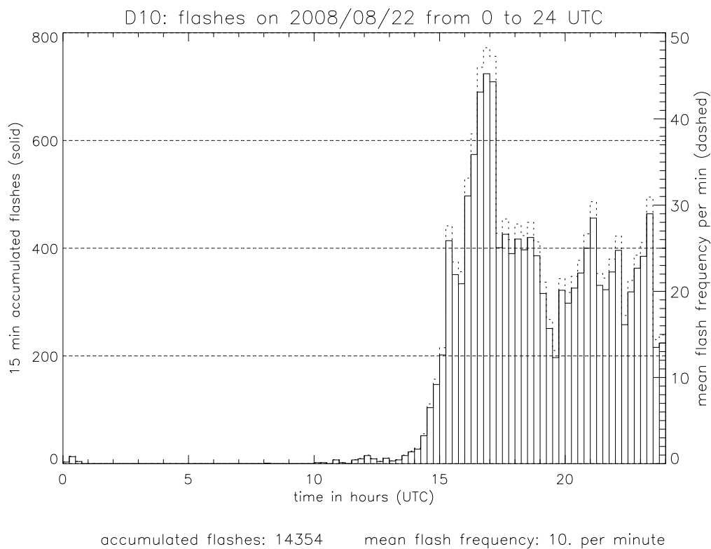
Figure 6.3: Histogram plots of observed lightning activity (a) and simulated lightning activity using the D10 scheme (b). Solid lines represent the 15-min accumulated flashes, and dashed lines represent the flash rate per minute.
