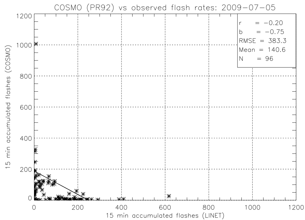
Figure 6.15: Correlation of the temporal evolution of the lightning activity based on LINET flashes and on the simulation using the PR92 parameterization. Two data points of 1,200 flashes per 15 min were omitted in the plot to ensure readability.
