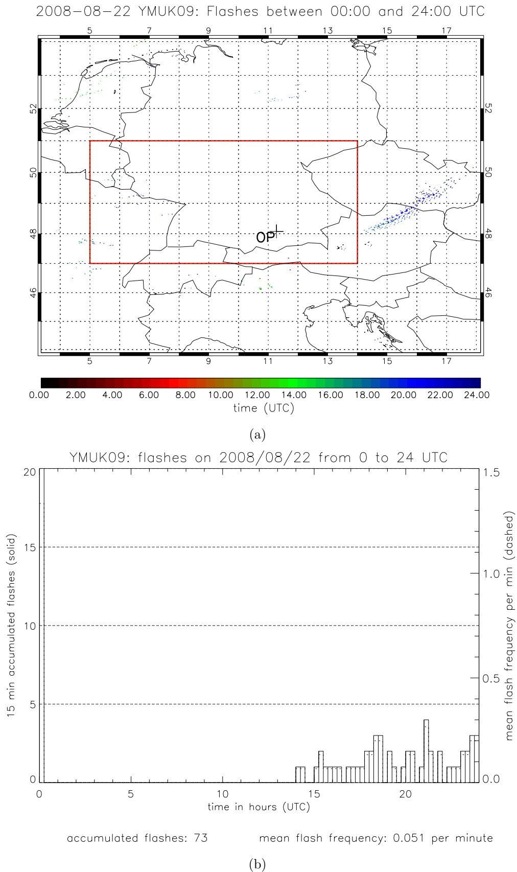
Figure 6.7: (a) Overview of the simulated lightning activity based on the YMUK09 parameterization, as in Fig. 6.2(b). (b) Histogram plot showing the temporal evolution of the lightning activity, based on YMUK09.
