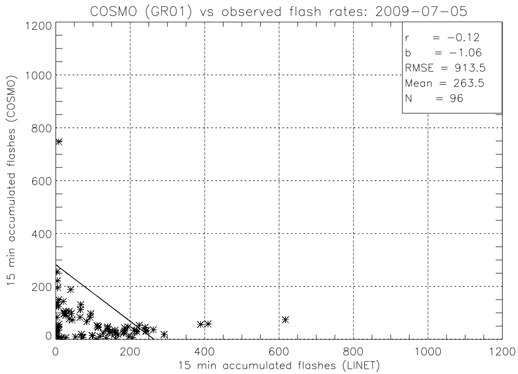
Figure 6.19: Correlation of the temporal evolution of the lightning activity based on LINET flashes and on the simulation using the GR01 parameterization. Two data points in excess of 3,000 flashes in 15 minutes were omitted in the plot to ensure readability.
