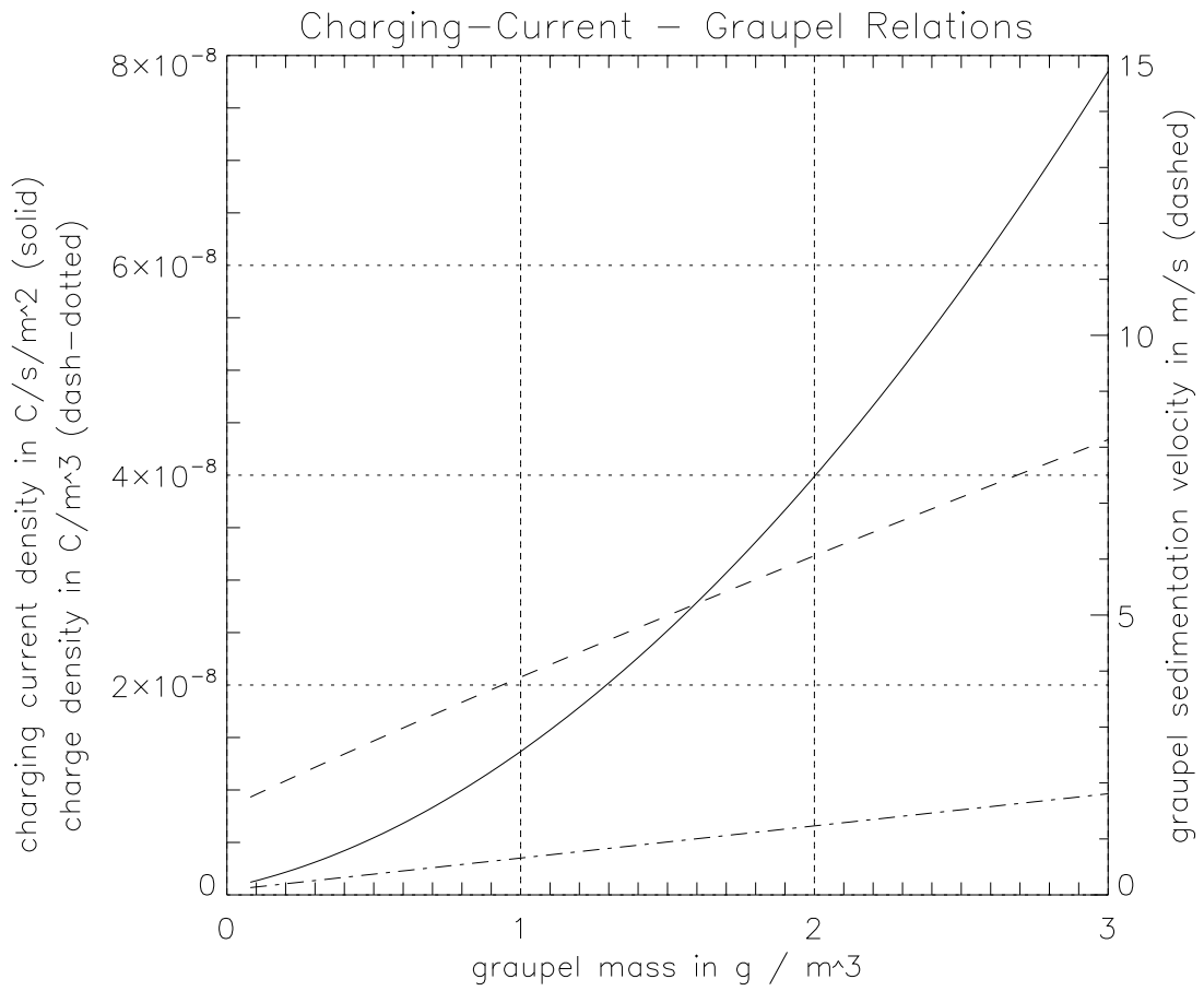
Figure 3.3: Parameterizations based on the graupel mass. The dashed line represents the terminal fall velocity of the graupel in ms^{-1} (right scale), the dash-dotted line represents the charge density in the generator current in Cm^{-3} , and the solid line represents the resulting generator current density.
