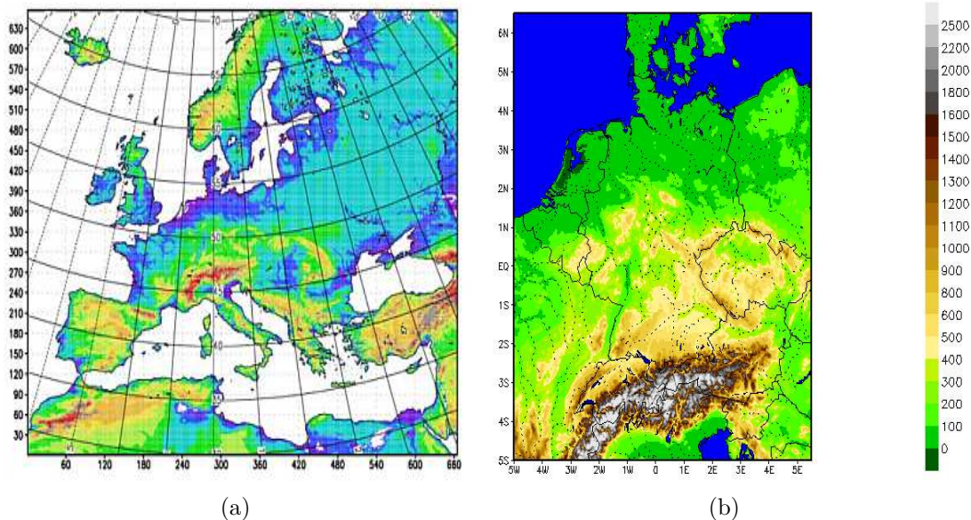
Figure B.1: COSMO-EU domain (a) and the COSMO-DE domain (b). Images courtesy of DWD.
