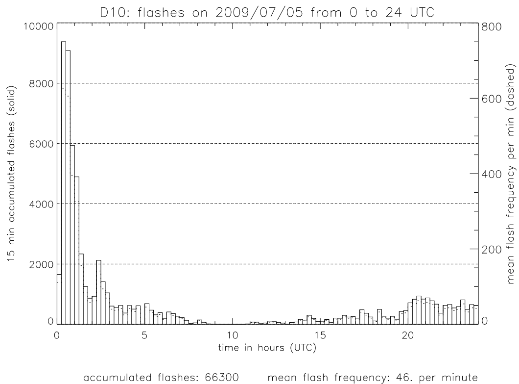
Figure 6.12: Histogram plots of observed lightning activity (a) and simulated lightning activity using the D10 scheme (b). Solid lines represent the 15-min accumulated flashes, and dashed lines represent the flash rate per minute.
