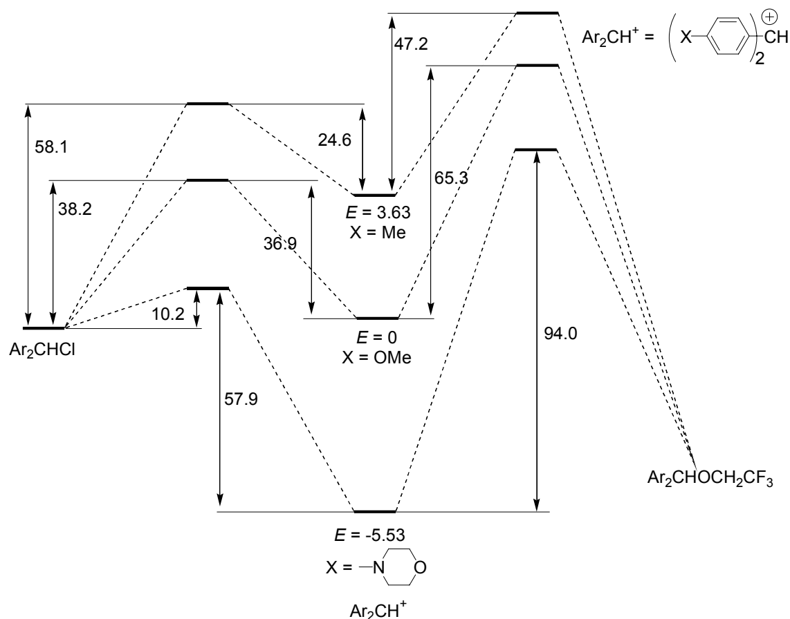
Figure 5.15: Free energy profiles for the solvolysis of various benzhydryl chlorides in TFE at 20 °C for the reactions of benzhydrylium ions with solvent and Cl - , at 25 °C for ionization. Unit is kJ mol -1 . N_f for Cl - in TFE was assumed as 6.1 from the rate constant of Ph 2 CHCl in 97/3 (w/w) TFE/Water (1.05 s -1 ) 21 with s_f = 1 .
