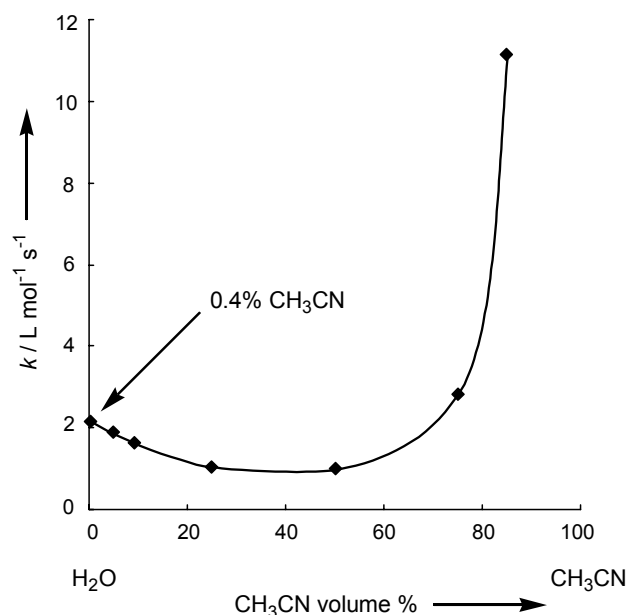
Figure 2.2: Solvent effect on the second-order rate constant of the reaction of (\text{lil})_2\text{CH}^+ with \text{OH}^- in acetonitrile–water mixtures (individual rate constants are given in Experimental Part). Because of the poor solubility of (\text{lil})_2\text{CH}^+\text{BF}_4^- , the rate constant in pure water cannot be measured.
