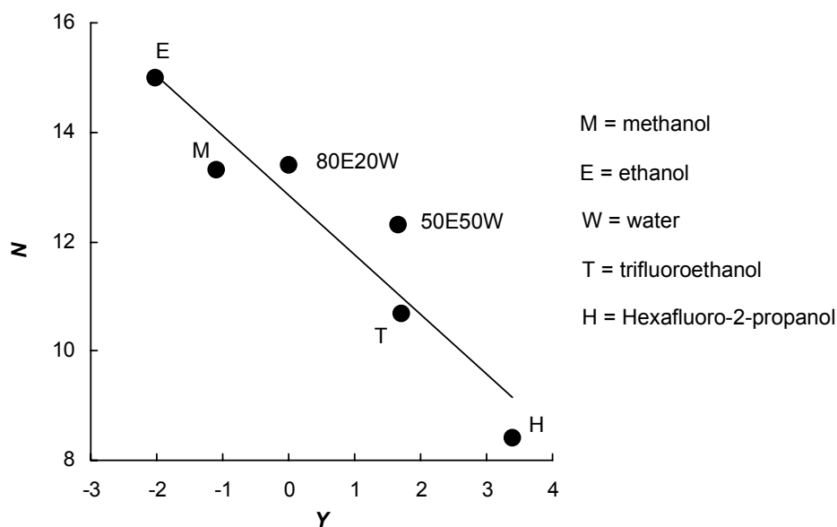
Figure 0.3: Correlation of N -parameters of Cl^- in several solvents with solvent ionizing power Y
