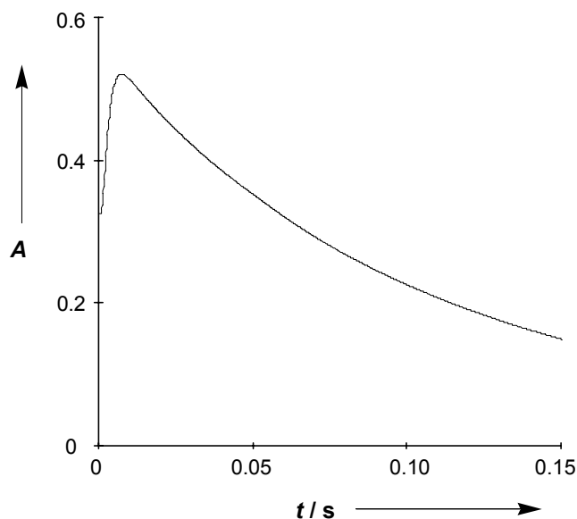
Figure 5.17: Generation and decay of the bis(4-methoxyphenyl)carbenium ion ((ani) 2 CH + ) observed after dissolving chloro-bis(4-methoxyphenyl)methane ((ani) 2 CHCl) in 20/80 (v/v) TFE/CH 3 CN containing 1.0 M of LiClO 4 .
