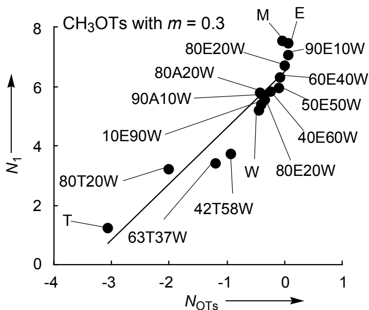
Figure 3.7: Relationship between nucleophilicity parameters N_1 and N_{OTs} from methyl tosylate. Mixtures of solvents are given as (v/v), solvents: M = methanol, E = ethanol, W = water, T = trifluoroethanol, A = acetone. Details are shown in Table 3.9.
