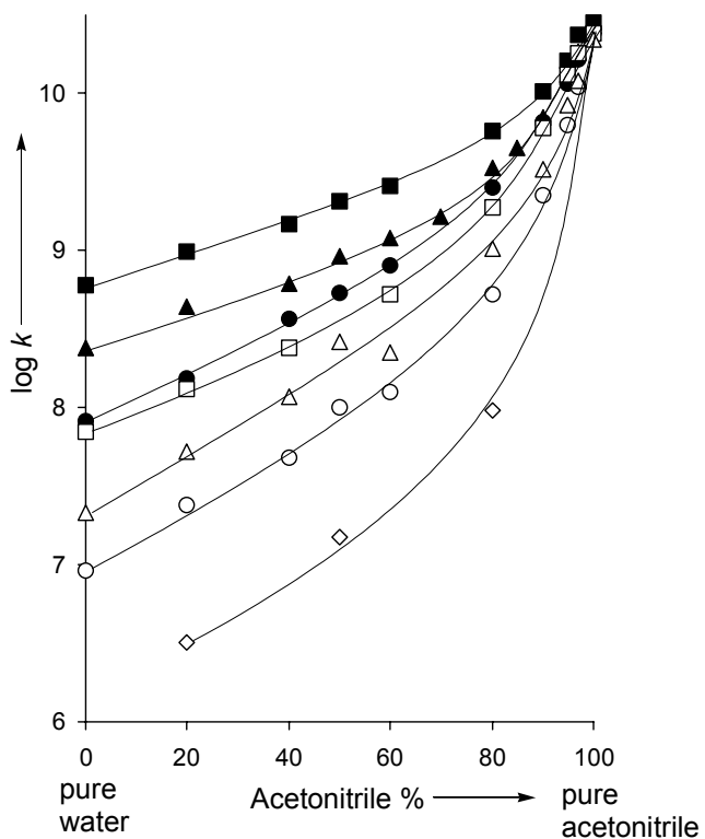
Figure 0.2: Variations in rate constants for the combinations of bromide anion and chloride anion with benzhydrylium ions in aqueous acetonitrile.
