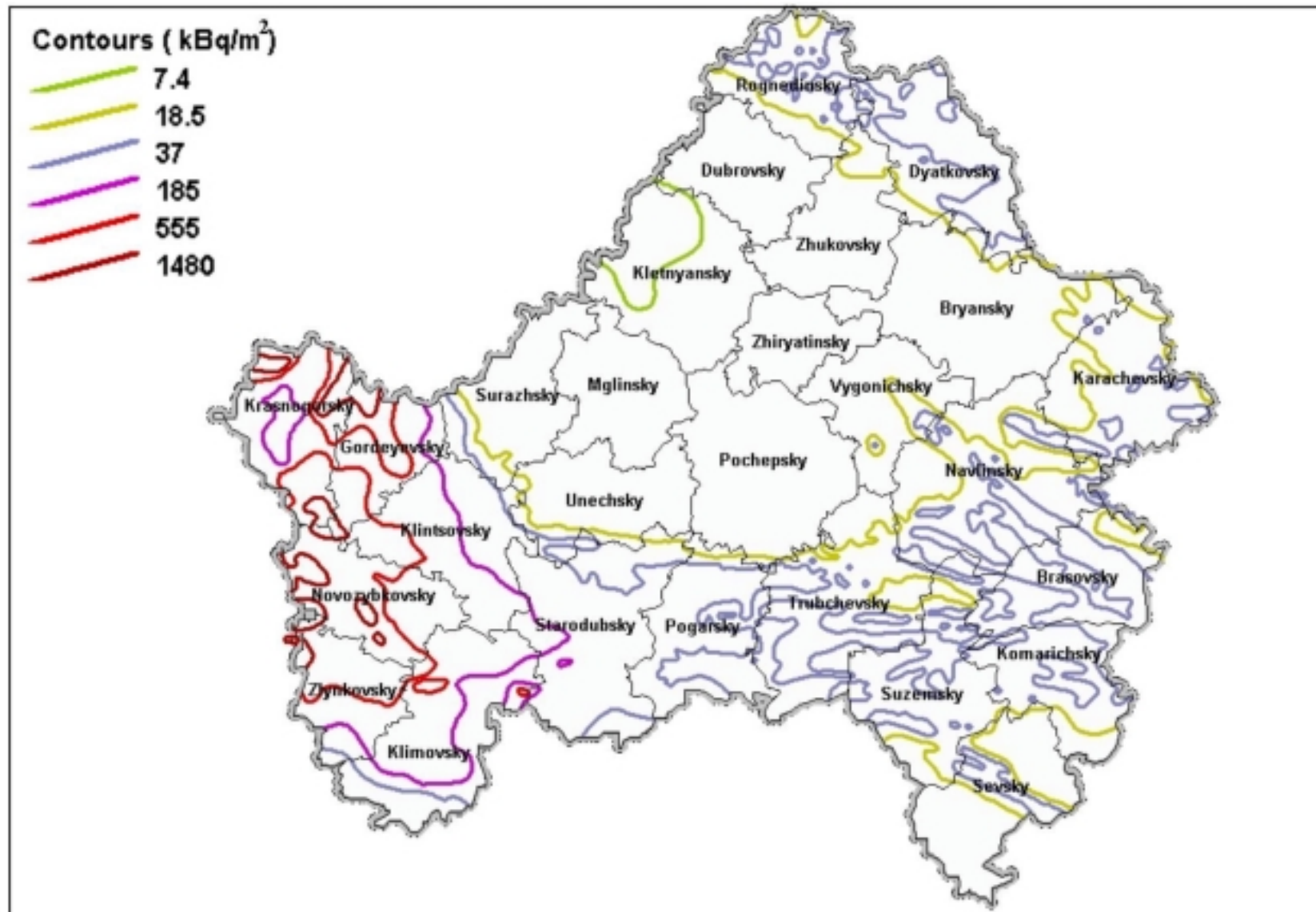
Fig 2.1 Official average density of ^{137}\text{Cs} contamination of the Bryansk oblast [MER 96]
