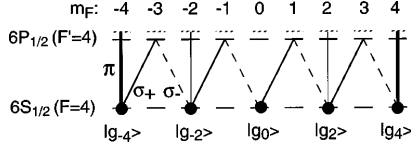
FIG. 2. Scheme of relevant levels of the cesium atom.
