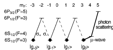
FIG. 2. Scheme of relevant levels of the cesium atom.
