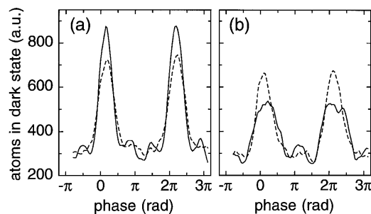
FIG. 3. Typical multiple beam interference fringes as a function of the phase of the second Ramsey pulse. (a) Signal without (solid line) and with an applied 9\text{-}\mu\text{s} -long optical pulse scattering photons from the path in m_F = 3 (dashed line). (b) In addition, a phase shift of \pi is applied to the path in m_F = 3 . Again, both spectra without (solid line) and with (dashed line) scattering of photons are shown. The principle maxima are slightly shifted from 0 and 2\pi , since the frequency difference of the optical Ramsey beams does not exactly match the Zeeman splitting of the magnetic sublevels.
