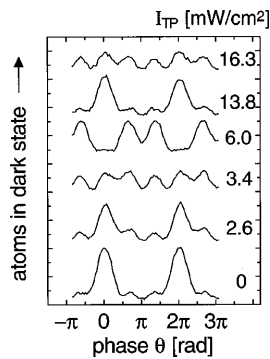
FIG. 5. Interference signal for different intensities I_{TP} as a function of the phase of the second projection pulse for an F=3 to F'=3 transition.
