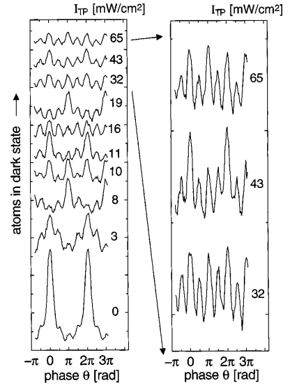
FIG. 4. Interference signals for an F=4 to F'=4 transition as a function of the phase of the second Ramsey pulse for different intensities I_{TP} . The three spectra with highest intensities are also shown on the right-hand side on an expanded scale.
