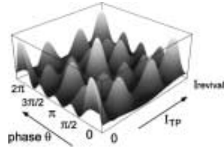
FIG. 3. Calculated interference signal for an F=4 to F'=4 transition as function of both the phase of the second Ramsey pulse \theta and the tensor polarizing beam intensity I_{TP} . The vertical scale gives the ratio |\langle \varphi_d(T) | \varphi_d(0) \rangle|^2 of atoms in the dark state after the pulses to those initially in that state.
