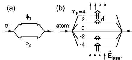
FIG. 1. Schematics of electric Aharonov-Bohm experiments (a) with electrons and two interfering paths and (b) with neutral atoms and five interfering paths.
