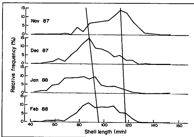
Fig. 1. Growth curve fitted to the 1987-1988 Sadh combined sexes abalone length frequency data with L_{\infty} = 137 mm SL, K = 0.75 \text{ year}^{-1} and t_0 = 0.73 \text{ year}^{-1} .
