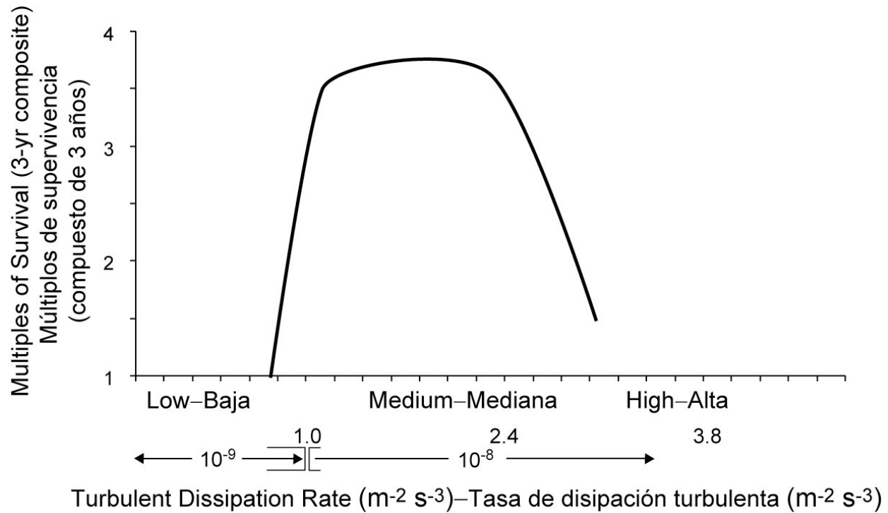
FIGURE 14. The relationship between microturbulence (estimated as the turbulent dissipation rate) and survival of yellowfin larvae during the first week of feeding in the laboratory. The survival curve is a smoothed, composite curve representing the mean survival estimated during 4 trials over 3 years.
